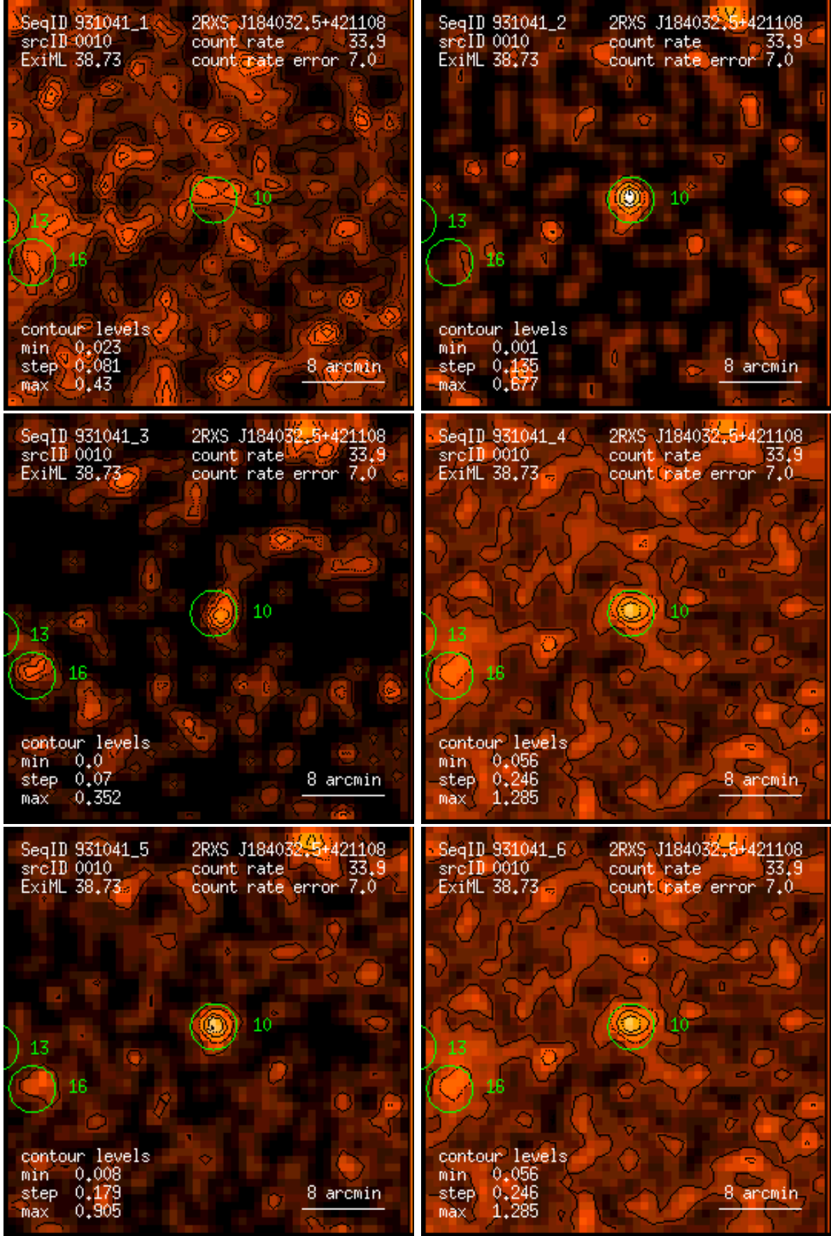
Figure 10: RASS 931041: detection 0010: band rate images, Gaussian filter: (1) PSPC channels 11 – 41, (2) 52 – 90, (3) 91 – 201, (4) 11 – 235, (5) 52 – 201, (6) 11 – 201. Broad band rates in counts/ks. Band rate contour levels in counts/ks/arcmin 2 .
