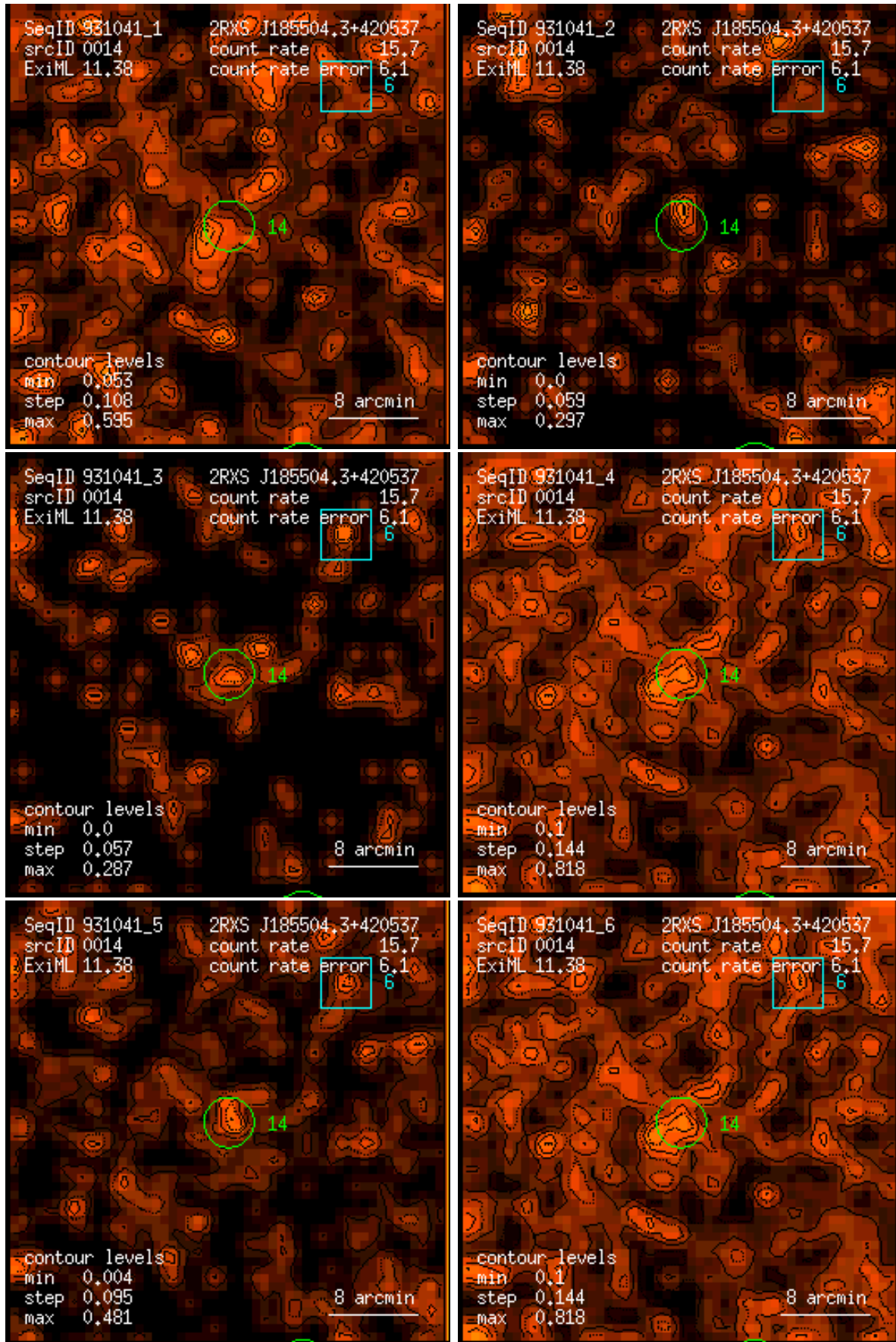
Figure 14: RASS 931041: detection 0014: band rate images, Gaussian filter: (1) PSPC channels 11 – 41, (2) 52 – 90, (3) 91 – 201, (4) 11 – 235, (5) 52 – 201, (6) 11 – 201. Broad band rates in counts/ks. Band rate contour levels in counts/ks/arcmin 2 .
