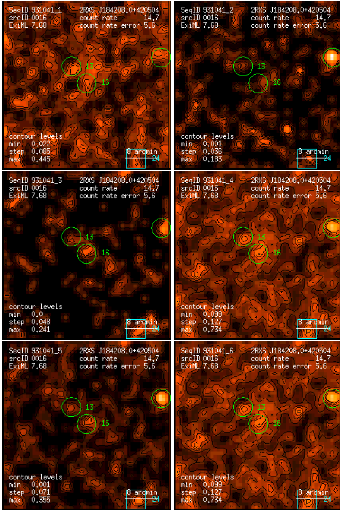
Figure 16: RASS 931041: detection 0016: band rate images, Gaussian filter: (1) PSPC channels 11 – 41, (2) 52 – 90, (3) 91 – 201, (4) 11 – 235, (5) 52 – 201, (6) 11 – 201. Broad band rates in counts/ks. Band rate contour levels in counts/ks/arcmin 2 .
