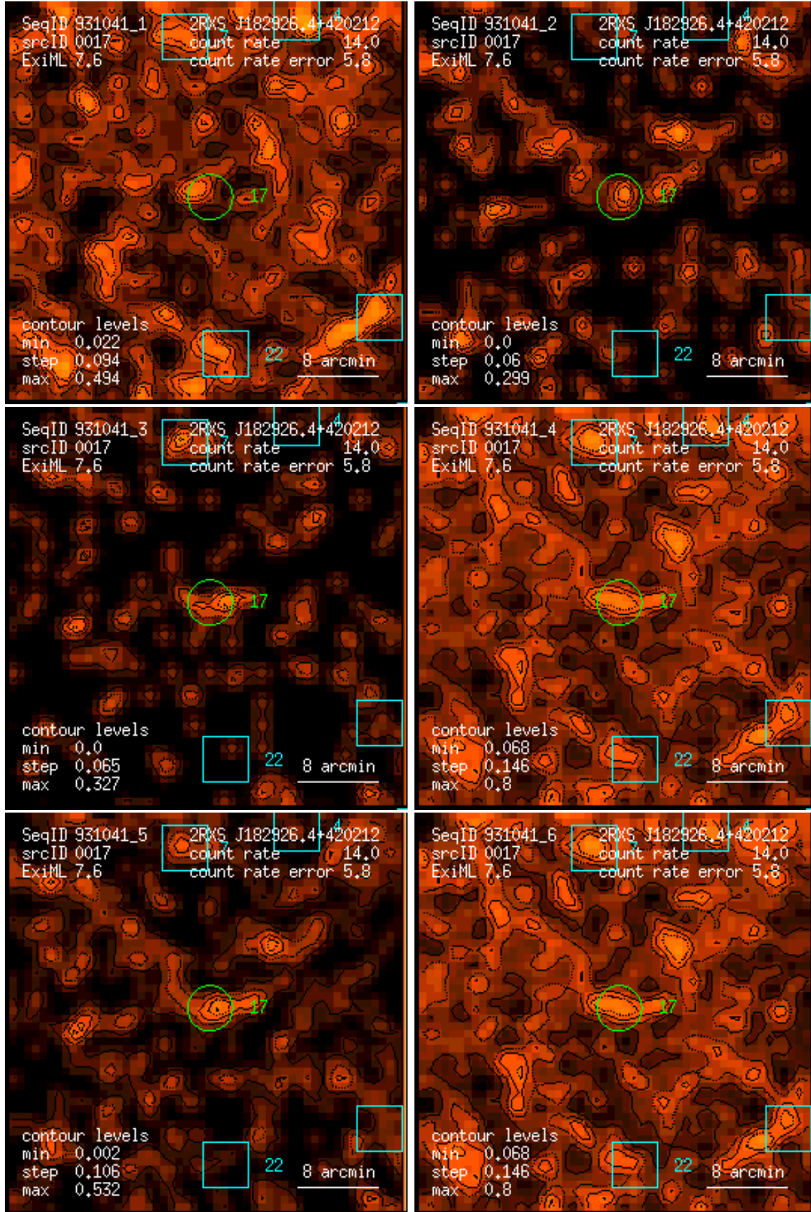
Figure 17: RASS 931041: detection 0017: band rate images, Gaussian filter: (1) PSPC channels 11 – 41, (2) 52 – 90, (3) 91 – 201, (4) 11 – 235, (5) 52 – 201, (6) 11 – 201. Broad band rates in counts/ks. Band rate contour levels in counts/ks/arcmin 2 .
