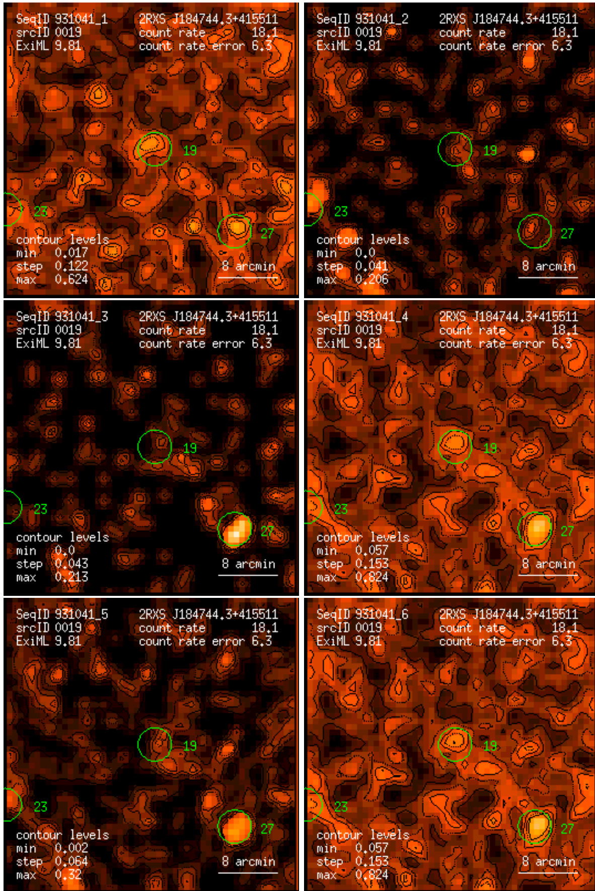
Figure 19: RASS 931041: detection 0019: band rate images, Gaussian filter: (1) PSPC channels 11 – 41, (2) 52 – 90, (3) 91 – 201, (4) 11 – 235, (5) 52 – 201, (6) 11 – 201. Broad band rates in counts/ks. Band rate contour levels in counts/ks/arcmin 2 .
