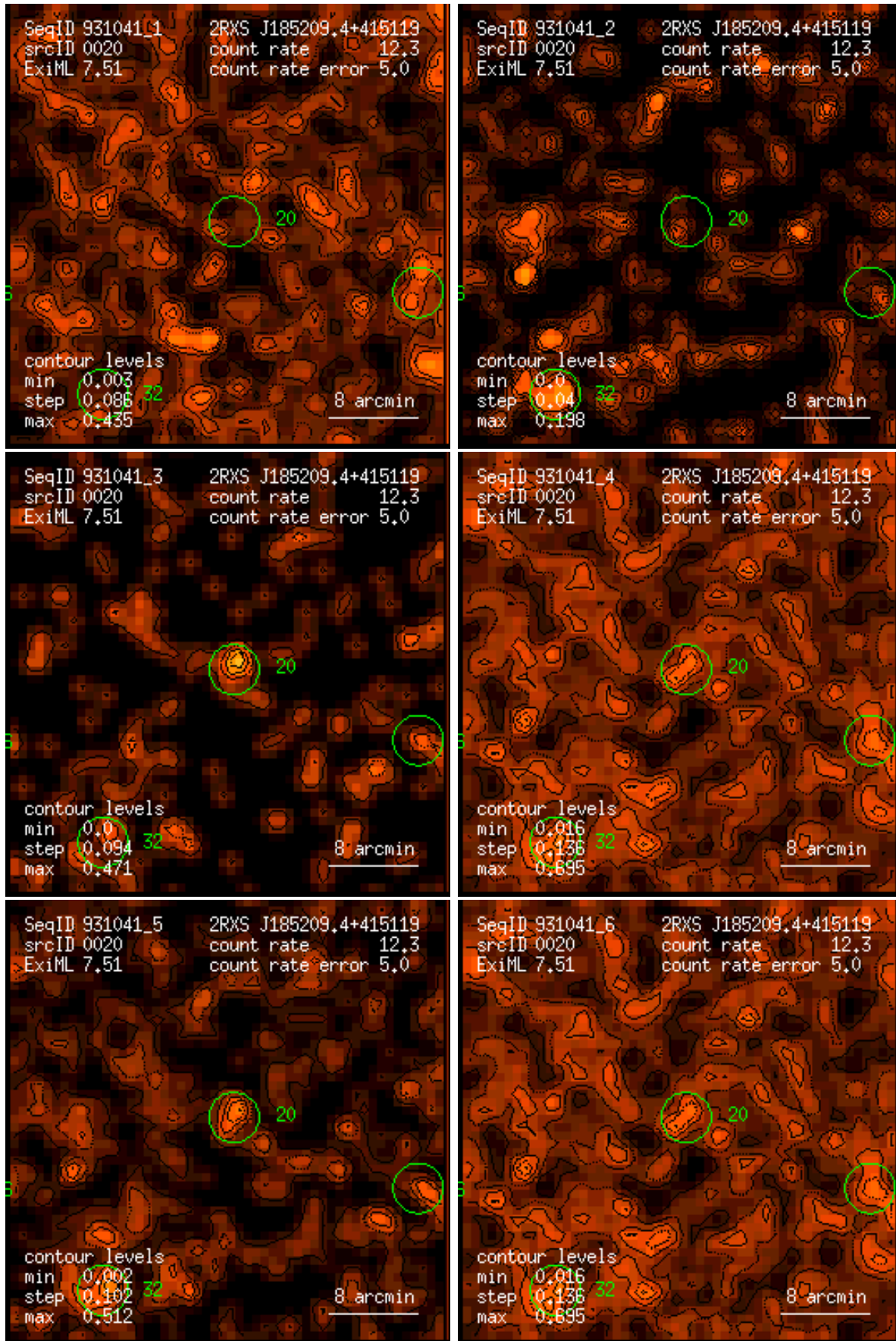
Figure 20: RASS 931041: detection 0020: band rate images, Gaussian filter: (1) PSPC channels 11 – 41, (2) 52 – 90, (3) 91 – 201, (4) 11 – 235, (5) 52 – 201, (6) 11 – 201. Broad band rates in counts/ks. Band rate contour levels in counts/ks/arcmin 2 .
