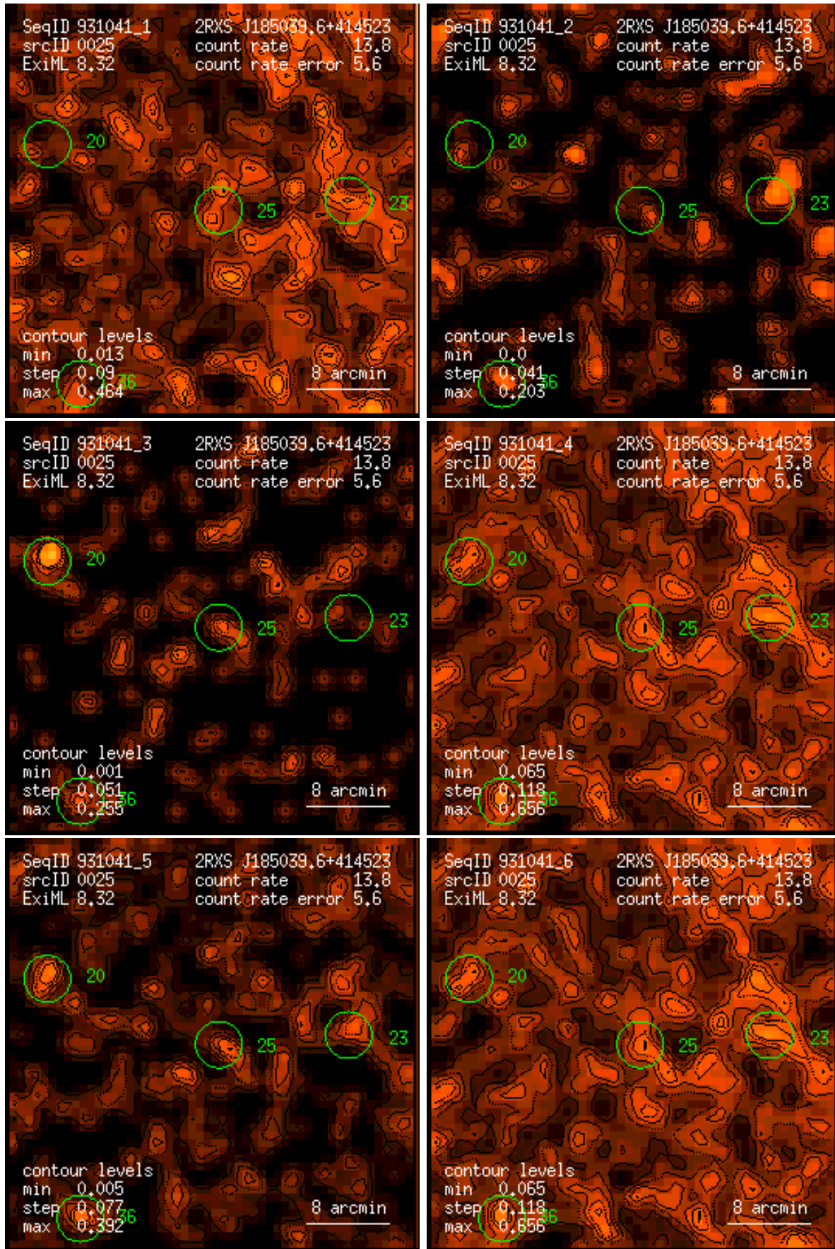
Figure 25: RASS 931041: detection 0025: band rate images, Gaussian filter: (1) PSPC channels 11 – 41, (2) 52 – 90, (3) 91 – 201, (4) 11 – 235, (5) 52 – 201, (6) 11 – 201. Broad band rates in counts/ks. Band rate contour levels in counts/ks/arcmin 2 .
