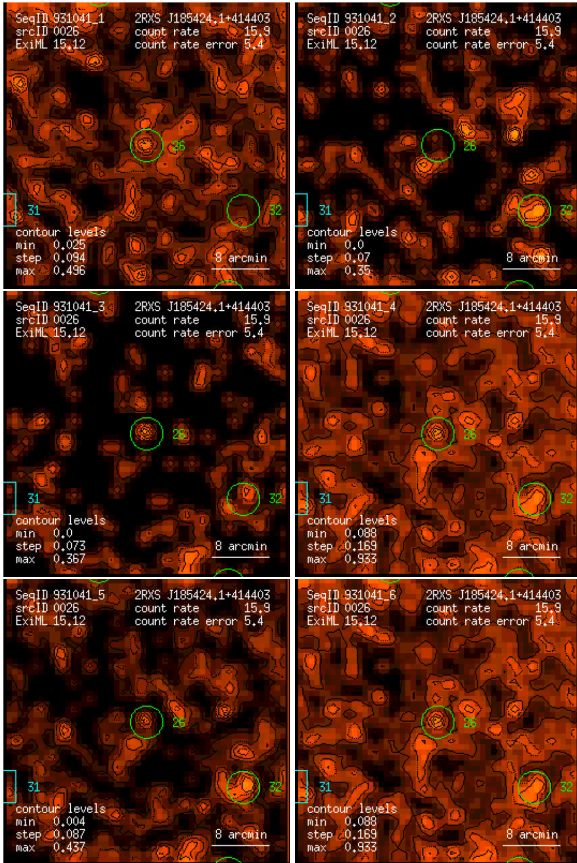
Figure 26: RASS 931041: detection 0026: band rate images, Gaussian filter: (1) PSPC channels 11 – 41, (2) 52 – 90, (3) 91 – 201, (4) 11 – 235, (5) 52 – 201, (6) 11 – 201. Broad band rates in counts/ks. Band rate contour levels in counts/ks/arcmin 2 .
