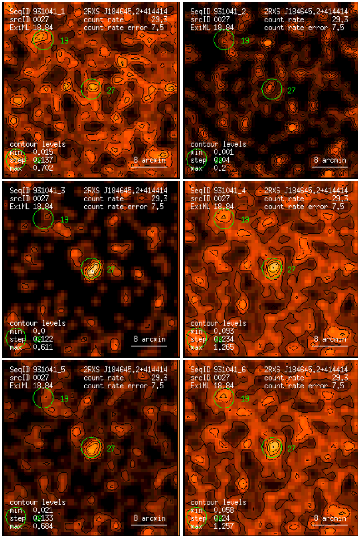
Figure 27: RASS 931041: detection 0027: band rate images, Gaussian filter: (1) PSPC channels 11 – 41, (2) 52 – 90, (3) 91 – 201, (4) 11 – 235, (5) 52 – 201, (6) 11 – 201. Broad band rates in counts/ks. Band rate contour levels in counts/ks/arcmin 2 .
