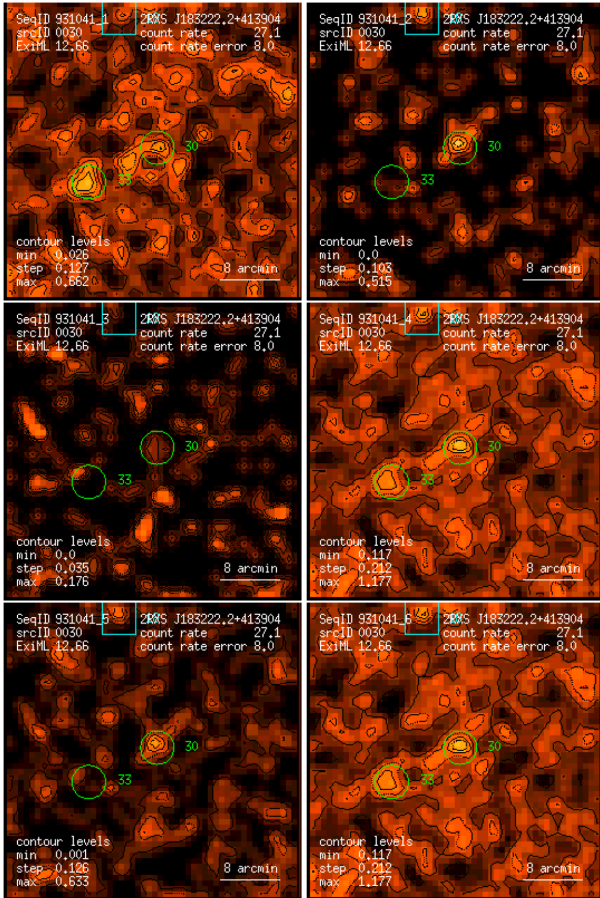
Figure 30: RASS 931041: detection 0030: band rate images, Gaussian filter: (1) PSPC channels 11 – 41, (2) 52 – 90, (3) 91 – 201, (4) 11 – 235, (5) 52 – 201, (6) 11 – 201. Broad band rates in counts/ks. Band rate contour levels in counts/ks/arcmin 2 .
