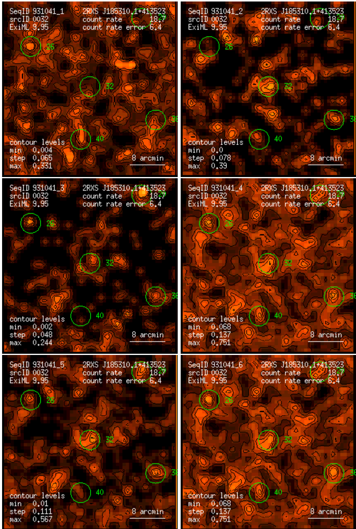
Figure 32: RASS 931041: detection 0032: band rate images, Gaussian filter: (1) PSPC channels 11 – 41, (2) 52 – 90, (3) 91 – 201, (4) 11 – 235, (5) 52 – 201, (6) 11 – 201. Broad band rates in counts/ks. Band rate contour levels in counts/ks/arcmin 2 .
