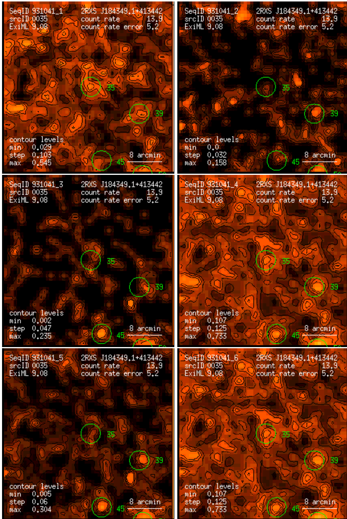
Figure 35: RASS 931041: detection 0035: band rate images, Gaussian filter: (1) PSPC channels 11 – 41, (2) 52 – 90, (3) 91 – 201, (4) 11 – 235, (5) 52 – 201, (6) 11 – 201. Broad band rates in counts/ks. Band rate contour levels in counts/ks/arcmin 2 .
