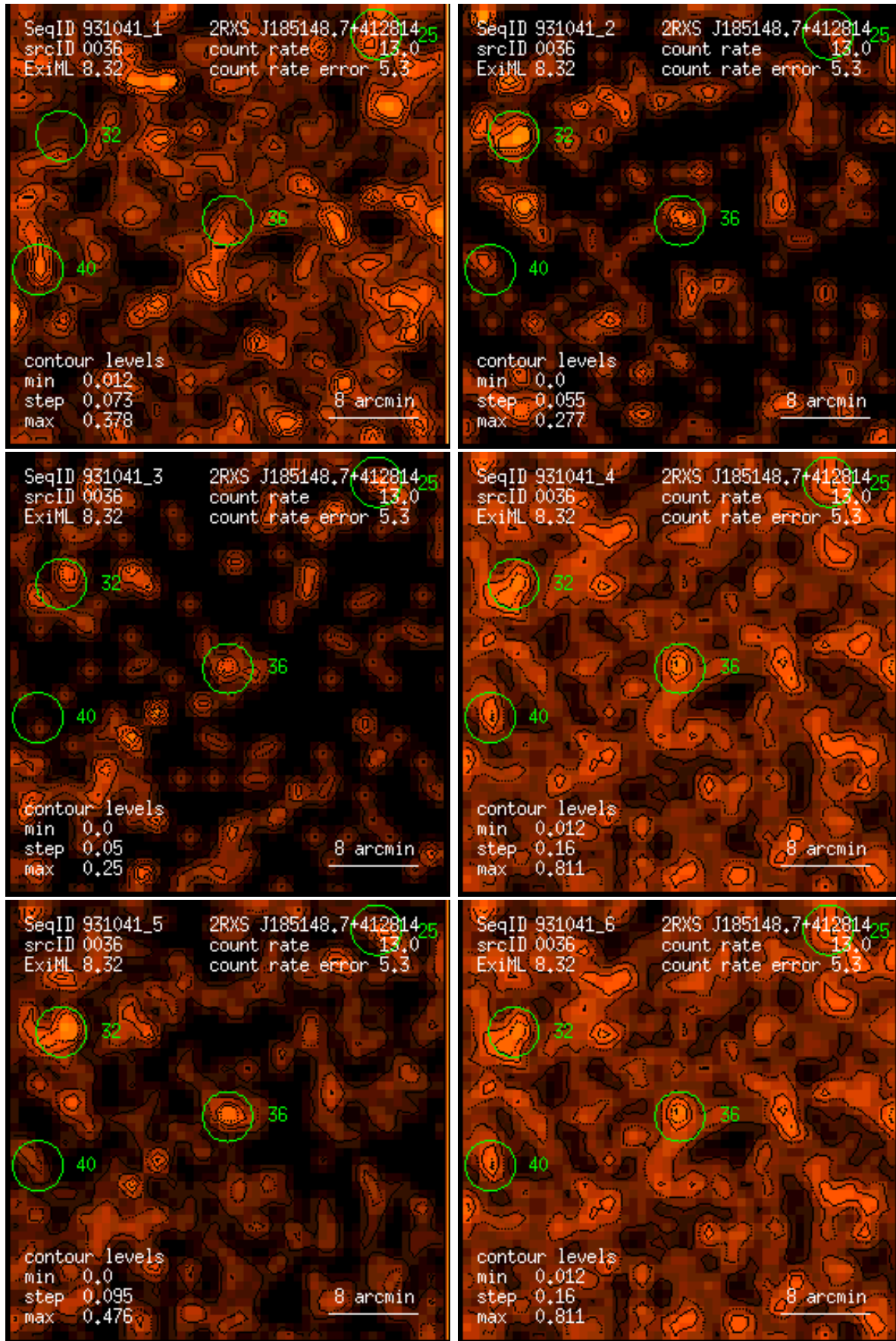
Figure 36: RASS 931041: detection 0036: band rate images, Gaussian filter: (1) PSPC channels 11 – 41, (2) 52 – 90, (3) 91 – 201, (4) 11 – 235, (5) 52 – 201, (6) 11 – 201. Broad band rates in counts/ks. Band rate contour levels in counts/ks/arcmin 2 .
