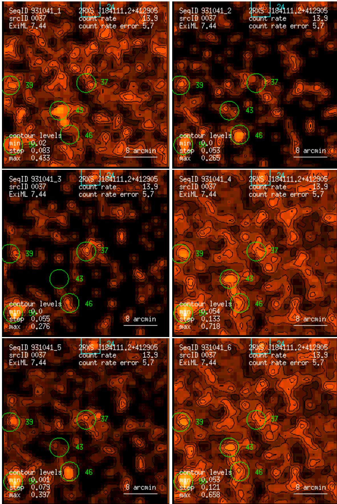
Figure 37: RASS 931041: detection 0037: band rate images, Gaussian filter: (1) PSPC channels 11 – 41, (2) 52 – 90, (3) 91 – 201, (4) 11 – 235, (5) 52 – 201, (6) 11 – 201. Broad band rates in counts/ks. Band rate contour levels in counts/ks/arcmin 2 .
