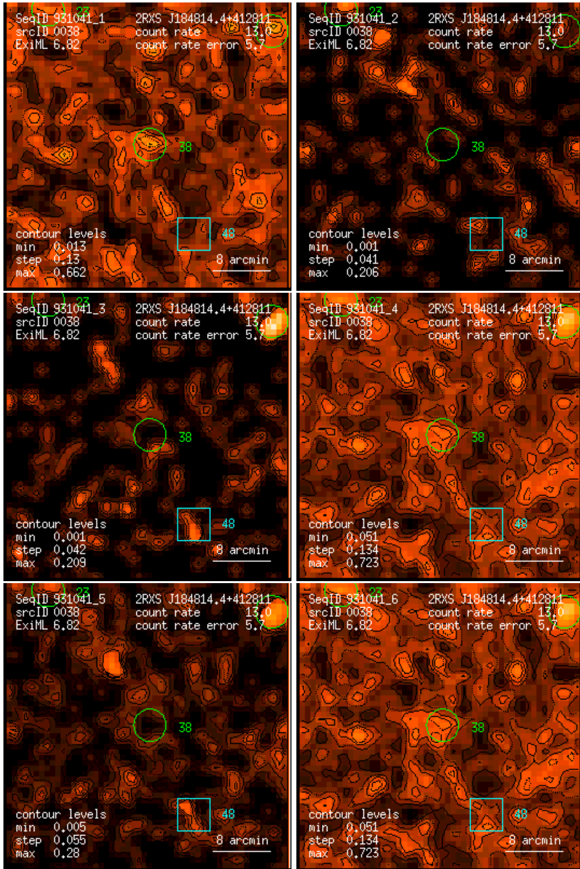
Figure 38: RASS 931041: detection 0038: band rate images, Gaussian filter: (1) PSPC channels 11 – 41, (2) 52 – 90, (3) 91 – 201, (4) 11 – 235, (5) 52 – 201, (6) 11 – 201. Broad band rates in counts/ks. Band rate contour levels in counts/ks/arcmin 2 .
