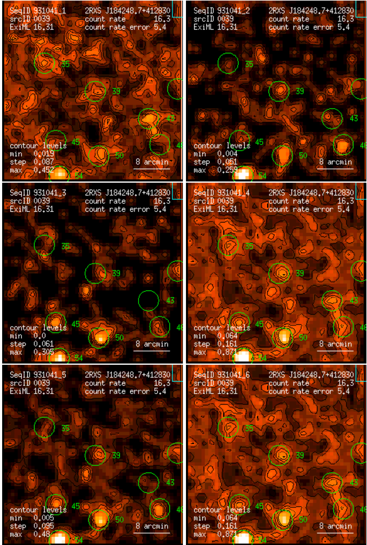
Figure 39: RASS 931041: detection 0039: band rate images, Gaussian filter: (1) PSPC channels 11 – 41, (2) 52 – 90, (3) 91 – 201, (4) 11 – 235, (5) 52 – 201, (6) 11 – 201. Broad band rates in counts/ks. Band rate contour levels in counts/ks/arcmin 2 .
