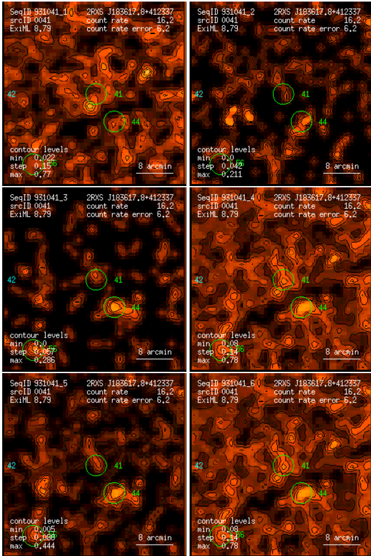
Figure 41: RASS 931041: detection 0041: band rate images, Gaussian filter: (1) PSPC channels 11 – 41, (2) 52 – 90, (3) 91 – 201, (4) 11 – 235, (5) 52 – 201, (6) 11 – 201. Broad band rates in counts/ks. Band rate contour levels in counts/ks/arcmin 2 .
