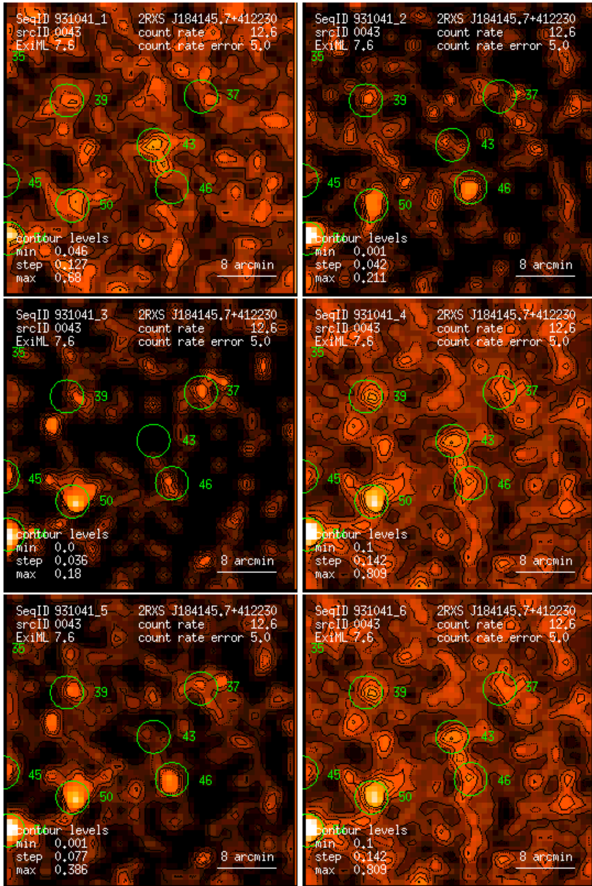
Figure 43: RASS 931041: detection 0043: band rate images, Gaussian filter: (1) PSPC channels 11 – 41, (2) 52 – 90, (3) 91 – 201, (4) 11 – 235, (5) 52 – 201, (6) 11 – 201. Broad band rates in counts/ks. Band rate contour levels in counts/ks/arcmin 2 .
