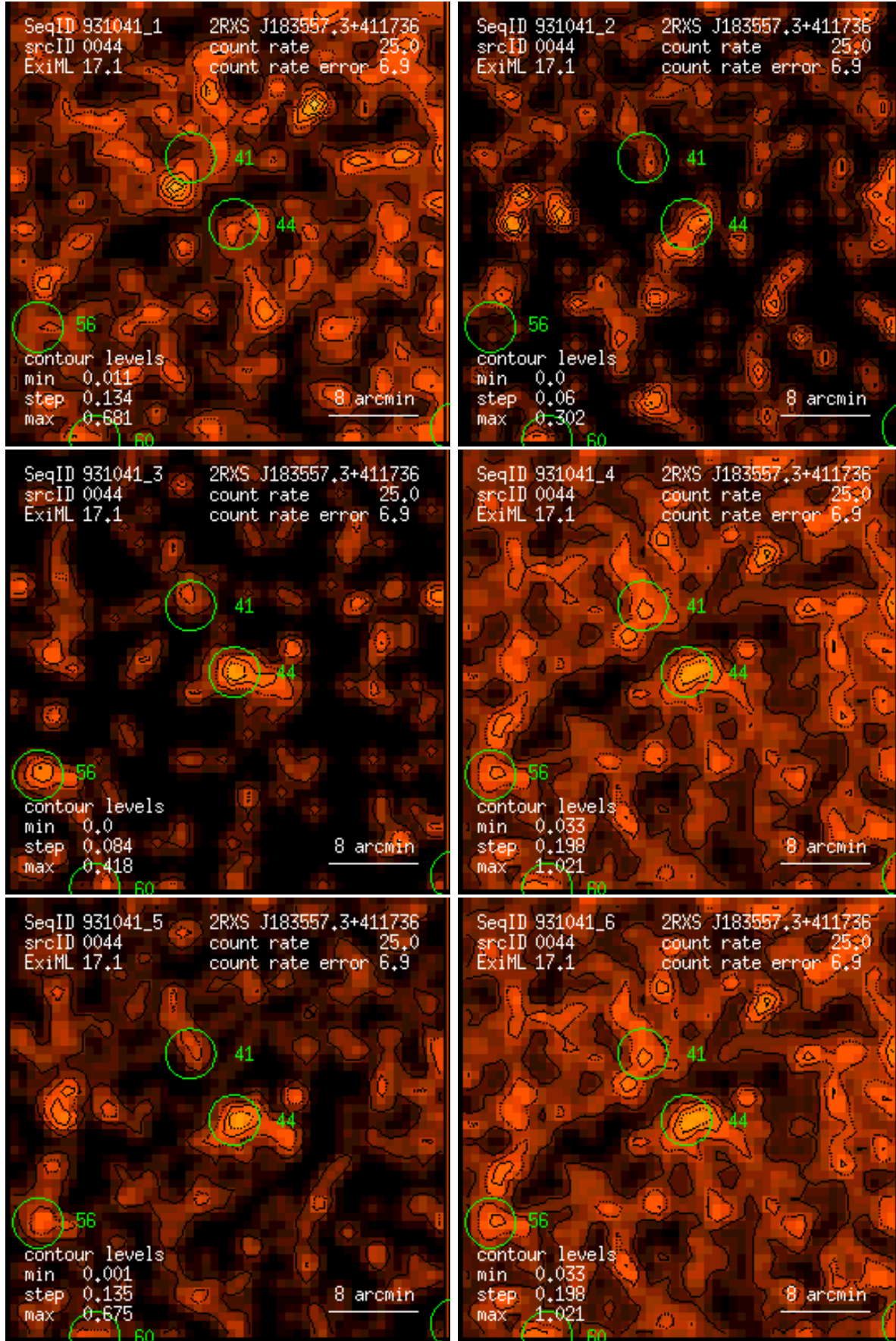
Figure 44: RASS 931041: detection 0044: band rate images, Gaussian filter: (1) PSPC channels 11 – 41, (2) 52 – 90, (3) 91 – 201, (4) 11 – 235, (5) 52 – 201, (6) 11 – 201. Broad band rates in counts/ks. Band rate contour levels in counts/ks/arcmin 2 .
