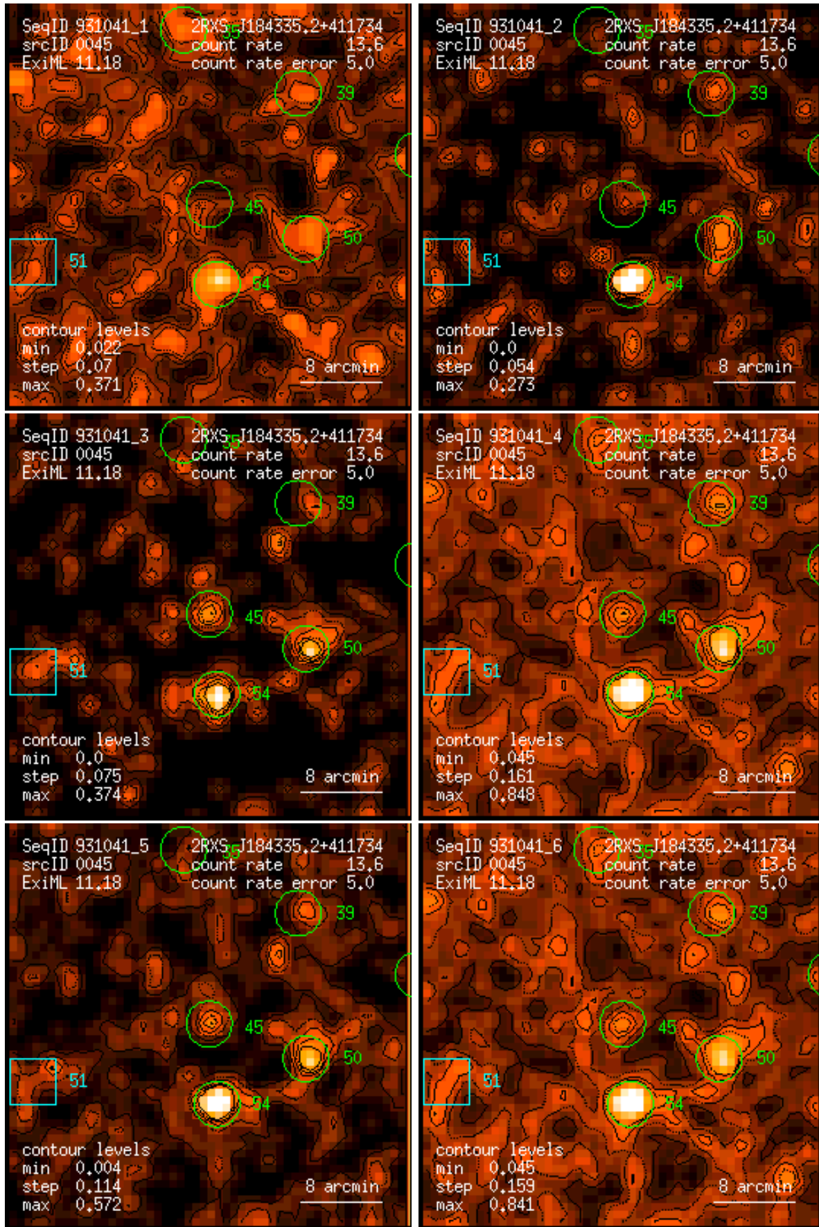
Figure 45: RASS 931041: detection 0045: band rate images, Gaussian filter: (1) PSPC channels 11 – 41, (2) 52 – 90, (3) 91 – 201, (4) 11 – 235, (5) 52 – 201, (6) 11 – 201. Broad band rates in counts/ks. Band rate contour levels in counts/ks/arcmin 2 .
