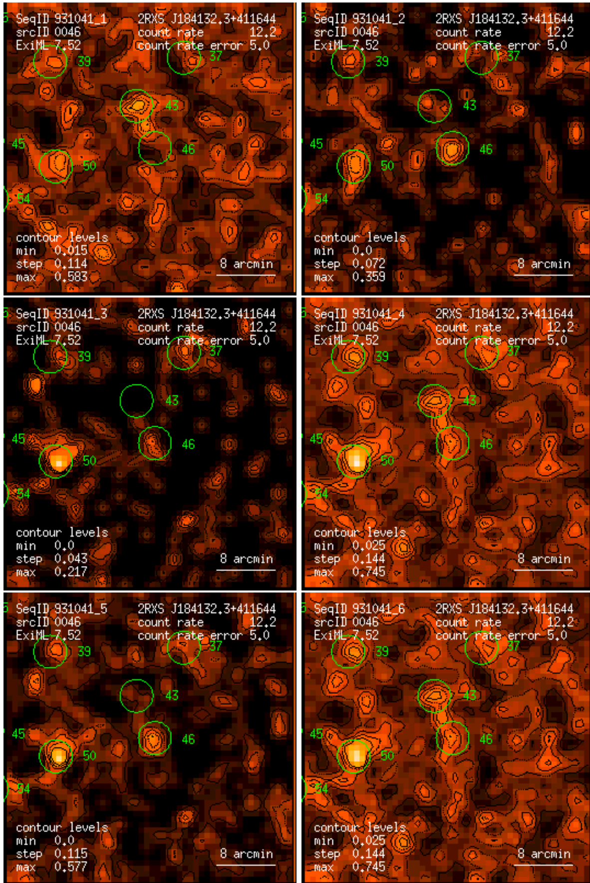
Figure 46: RASS 931041: detection 0046: band rate images, Gaussian filter: (1) PSPC channels 11 – 41, (2) 52 – 90, (3) 91 – 201, (4) 11 – 235, (5) 52 – 201, (6) 11 – 201. Broad band rates in counts/ks. Band rate contour levels in counts/ks/arcmin 2 .
