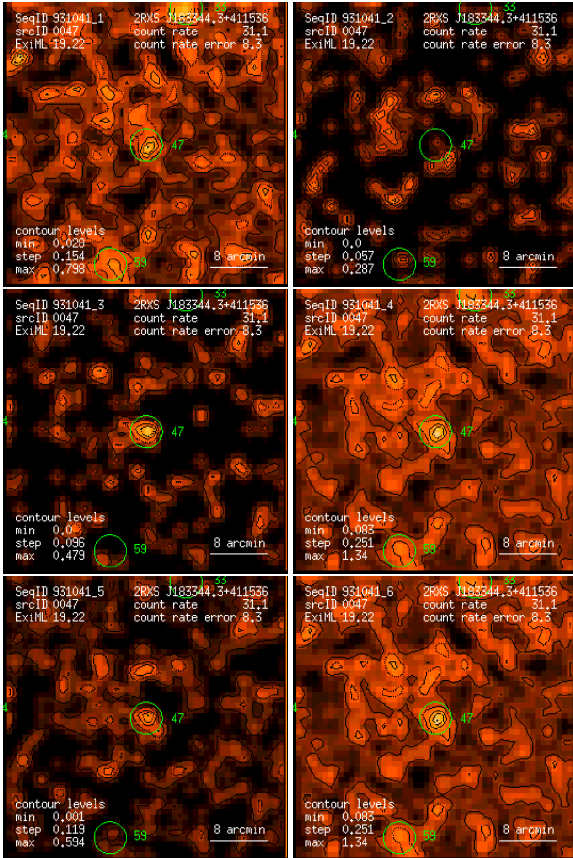
Figure 47: RASS 931041: detection 0047: band rate images, Gaussian filter: (1) PSPC channels 11 – 41, (2) 52 – 90, (3) 91 – 201, (4) 11 – 235, (5) 52 – 201, (6) 11 – 201. Broad band rates in counts/ks. Band rate contour levels in counts/ks/arcmin 2 .
