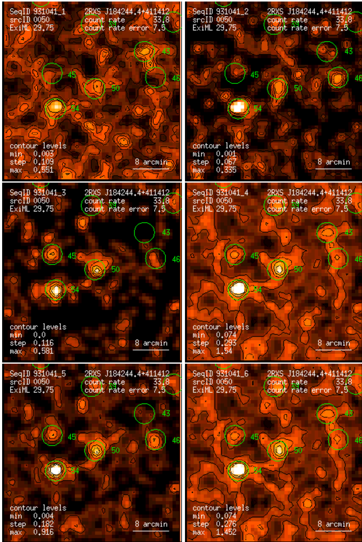
Figure 50: RASS 931041: detection 0050: band rate images, Gaussian filter: (1) PSPC channels 11 – 41, (2) 52 – 90, (3) 91 – 201, (4) 11 – 235, (5) 52 – 201, (6) 11 – 201. Broad band rates in counts/ks. Band rate contour levels in counts/ks/arcmin 2 .
