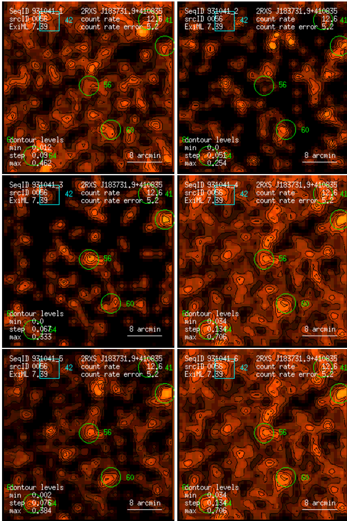
Figure 56: RASS 931041: detection 0056: band rate images, Gaussian filter: (1) PSPC channels 11 – 41, (2) 52 – 90, (3) 91 – 201, (4) 11 – 235, (5) 52 – 201, (6) 11 – 201. Broad band rates in counts/ks. Band rate contour levels in counts/ks/arcmin 2 .
