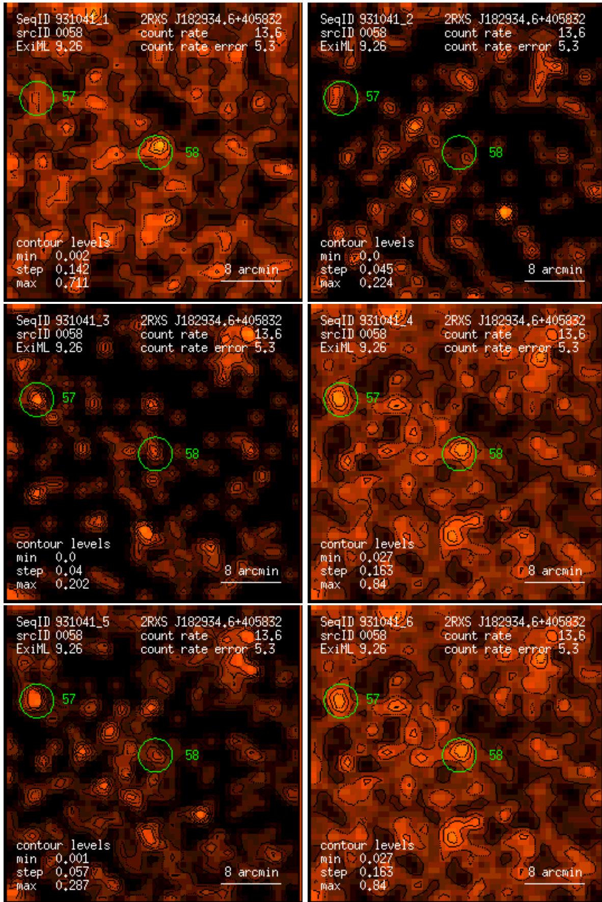
Figure 58: RASS 931041: detection 0058: band rate images, Gaussian filter: (1) PSPC channels 11 – 41, (2) 52 – 90, (3) 91 – 201, (4) 11 – 235, (5) 52 – 201, (6) 11 – 201. Broad band rates in counts/ks. Band rate contour levels in counts/ks/arcmin 2 .
