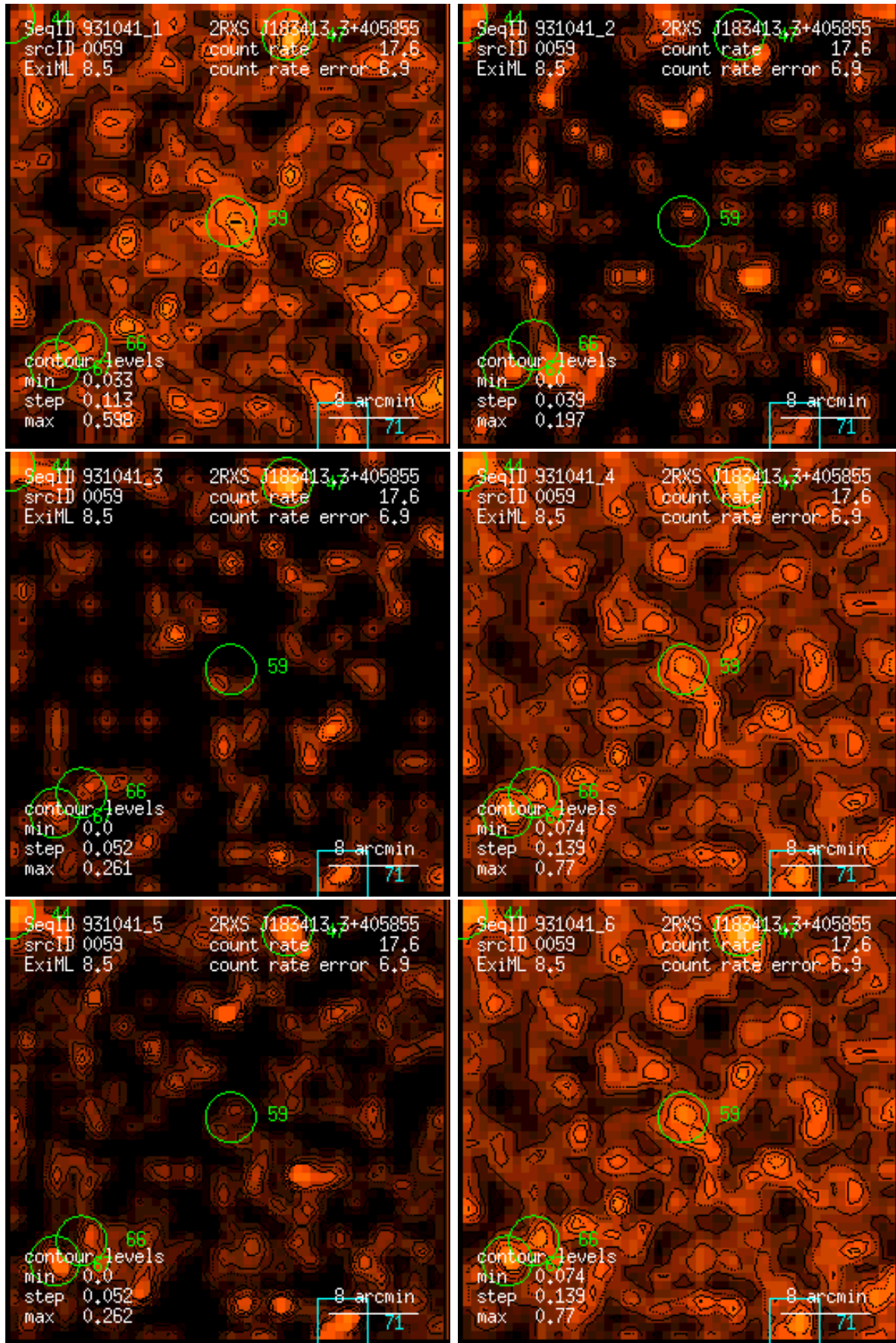
Figure 59: RASS 931041: detection 0059: band rate images, Gaussian filter: (1) PSPC channels 11 – 41, (2) 52 – 90, (3) 91 – 201, (4) 11 – 235, (5) 52 – 201, (6) 11 – 201. Broad band rates in counts/ks. Band rate contour levels in counts/ks/arcmin 2 .
