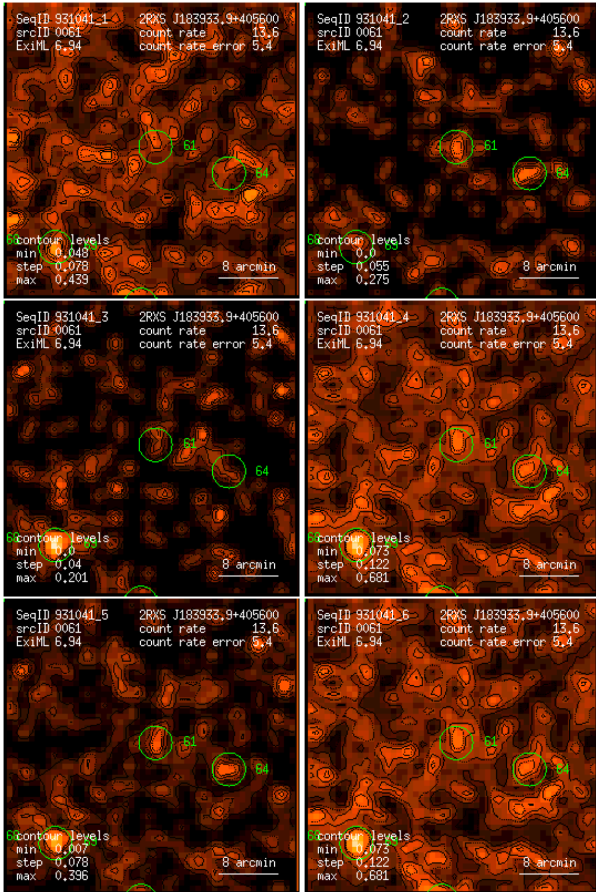
Figure 61: RASS 931041: detection 0061: band rate images, Gaussian filter: (1) PSPC channels 11 – 41, (2) 52 – 90, (3) 91 – 201, (4) 11 – 235, (5) 52 – 201, (6) 11 – 201. Broad band rates in counts/ks. Band rate contour levels in counts/ks/arcmin 2 .
