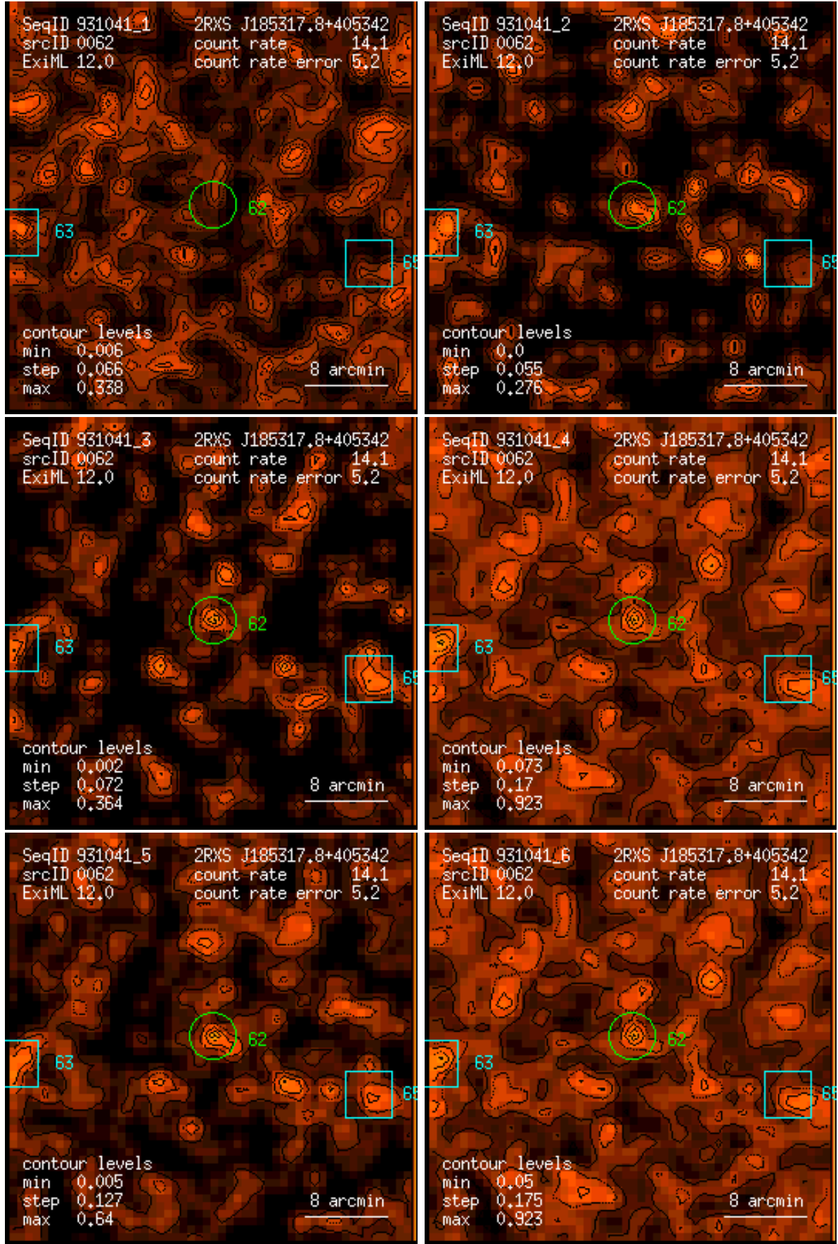
Figure 62: RASS 931041: detection 0062: band rate images, Gaussian filter: (1) PSPC channels 11 – 41, (2) 52 – 90, (3) 91 – 201, (4) 11 – 235, (5) 52 – 201, (6) 11 – 201. Broad band rates in counts/ks. Band rate contour levels in counts/ks/arcmin 2 .
