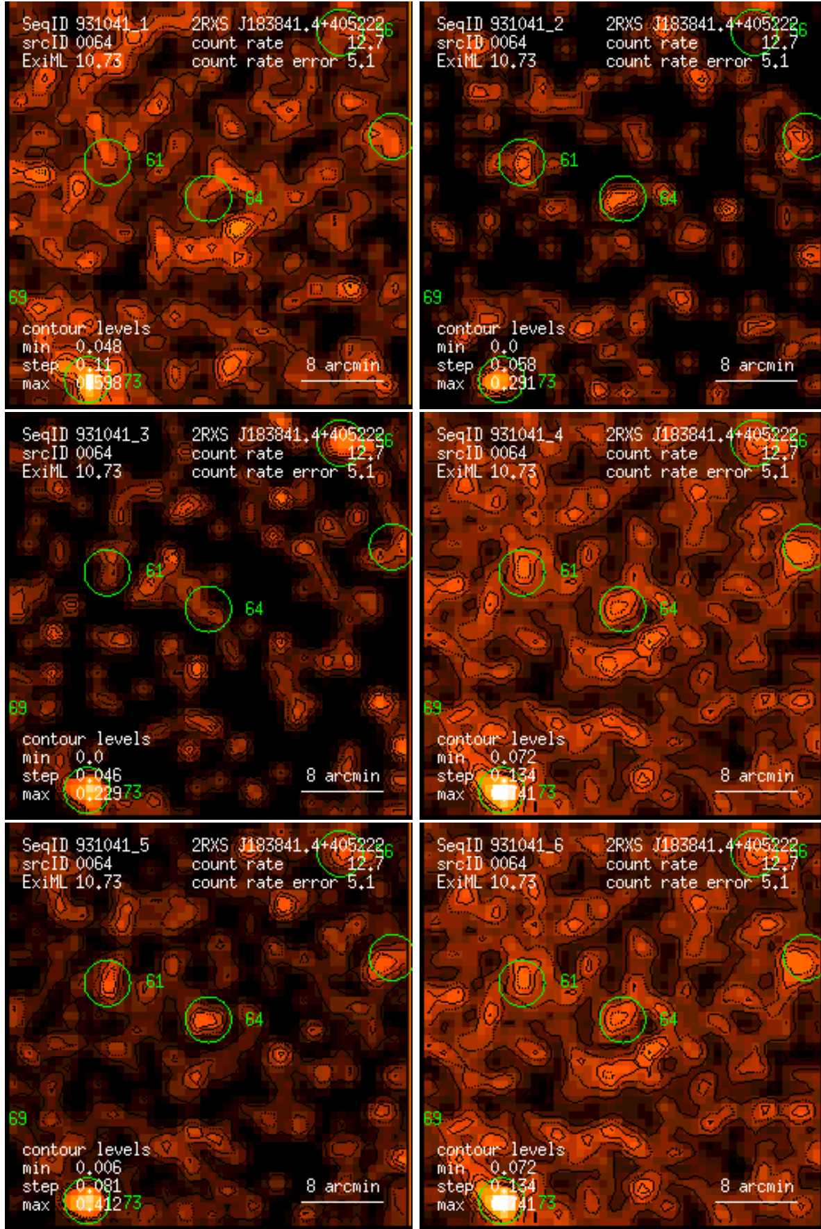
Figure 64: RASS 931041: detection 0064: band rate images, Gaussian filter: (1) PSPC channels 11 – 41, (2) 52 – 90, (3) 91 – 201, (4) 11 – 235, (5) 52 – 201, (6) 11 – 201. Broad band rates in counts/ks. Band rate contour levels in counts/ks/arcmin 2 .
