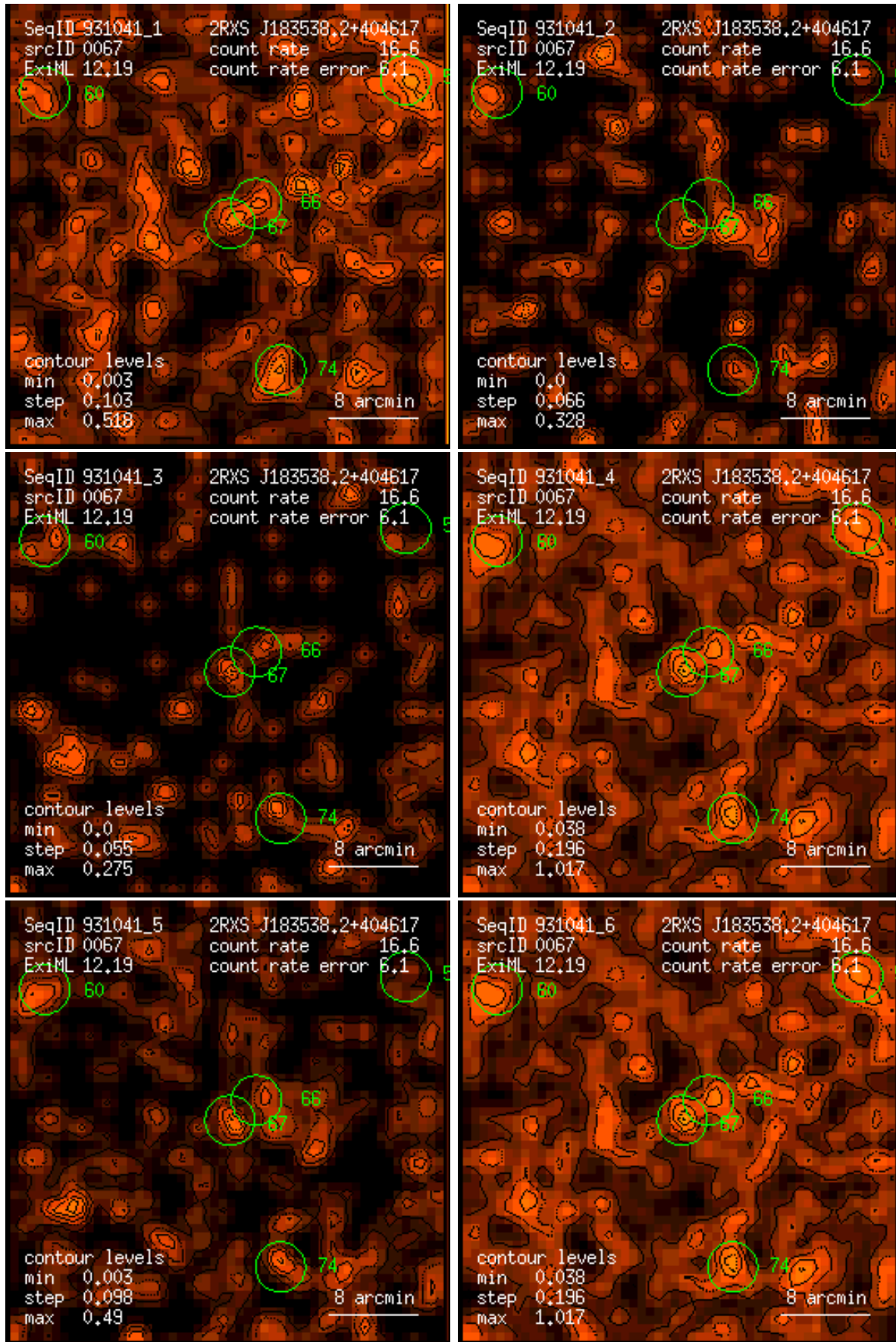
Figure 67: RASS 931041: detection 0067: band rate images, Gaussian filter: (1) PSPC channels 11 – 41, (2) 52 – 90, (3) 91 – 201, (4) 11 – 235, (5) 52 – 201, (6) 11 – 201. Broad band rates in counts/ks. Band rate contour levels in counts/ks/arcmin 2 .
