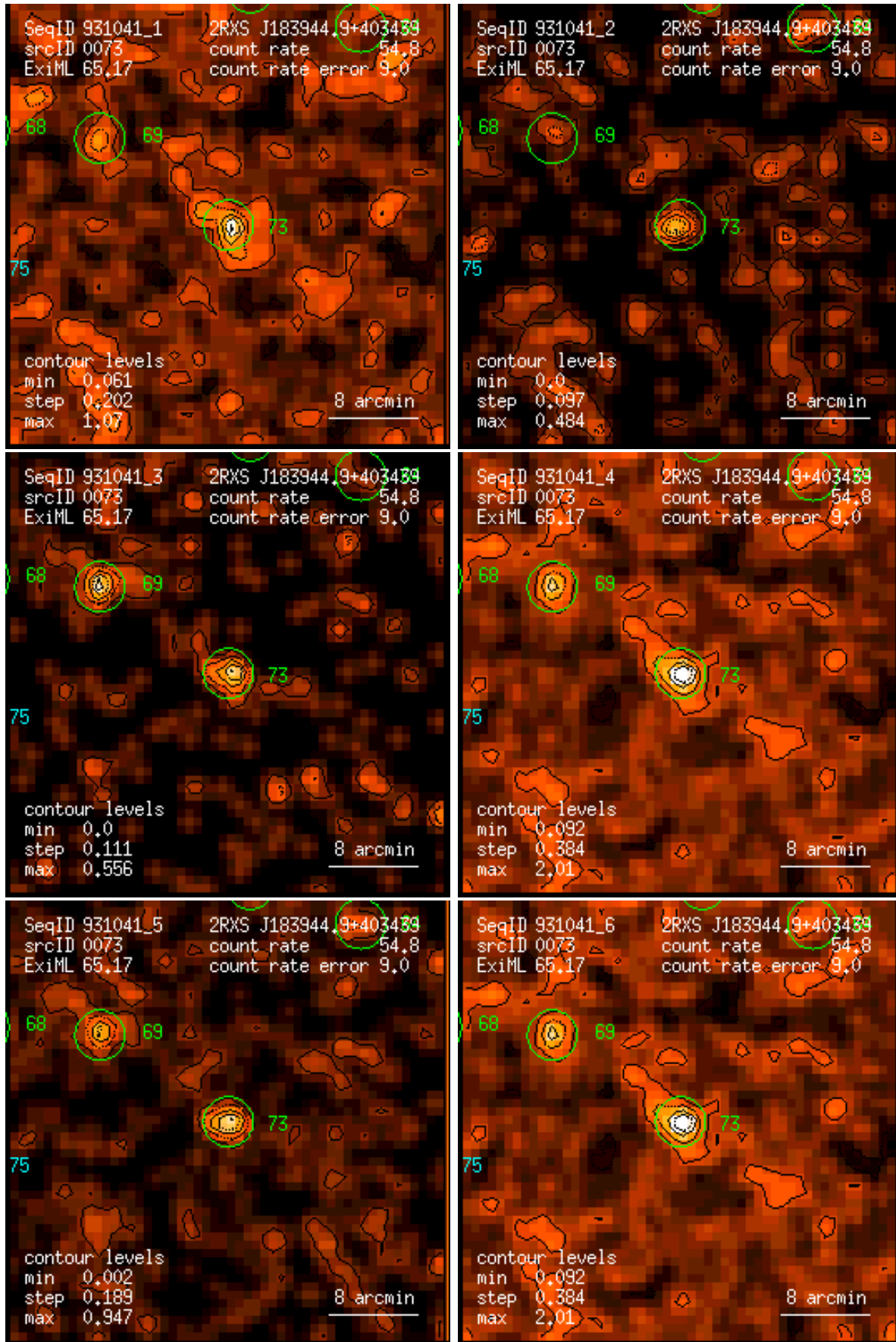
Figure 73: RASS 931041: detection 0073: band rate images, Gaussian filter: (1) PSPC channels 11 – 41, (2) 52 – 90, (3) 91 – 201, (4) 11 – 235, (5) 52 – 201, (6) 11 – 201. Broad band rates in counts/ks. Band rate contour levels in counts/ks/arcmin 2 .
