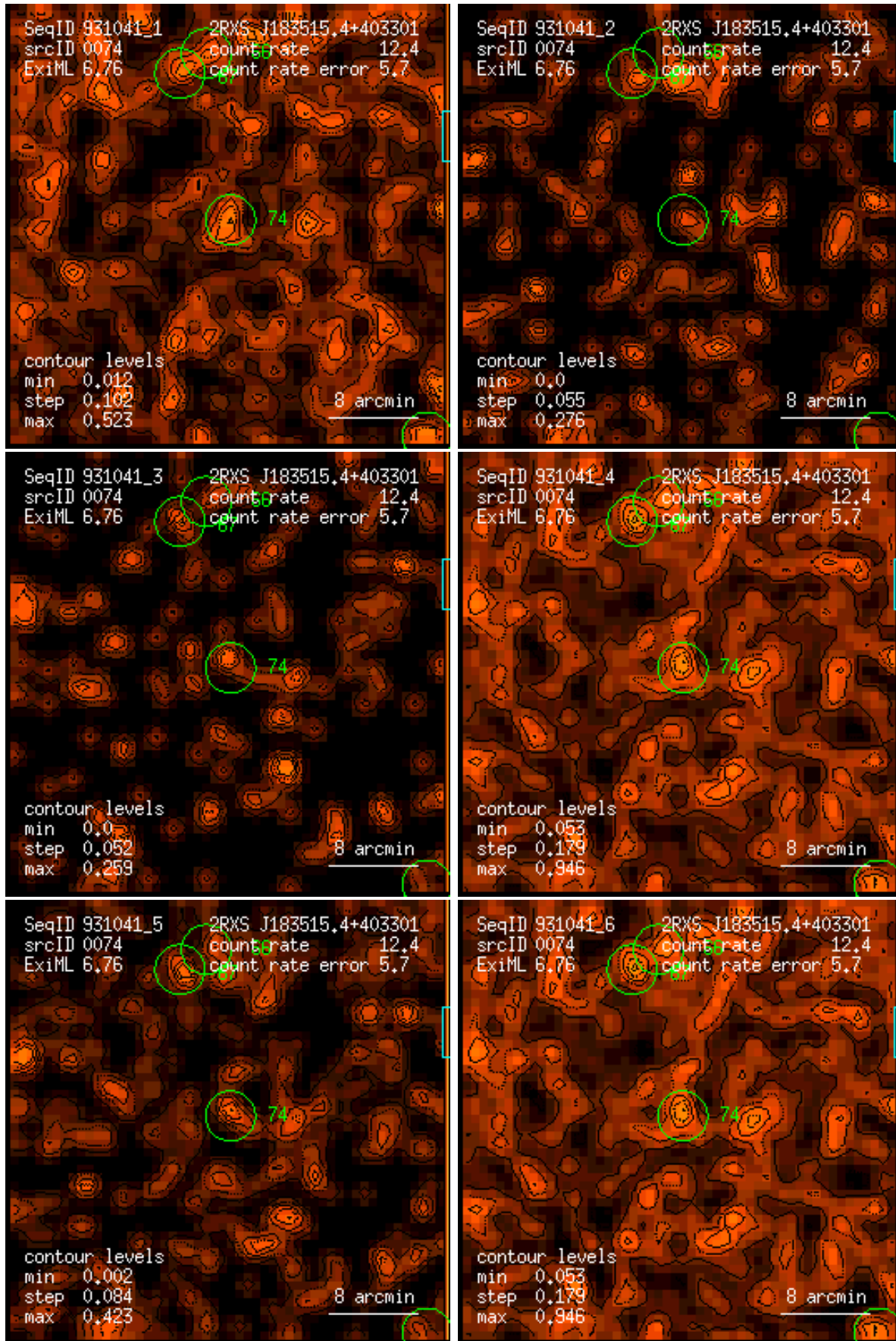
Figure 74: RASS 931041: detection 0074: band rate images, Gaussian filter: (1) PSPC channels 11 – 41, (2) 52 – 90, (3) 91 – 201, (4) 11 – 235, (5) 52 – 201, (6) 11 – 201. Broad band rates in counts/ks. Band rate contour levels in counts/ks/arcmin 2 .
