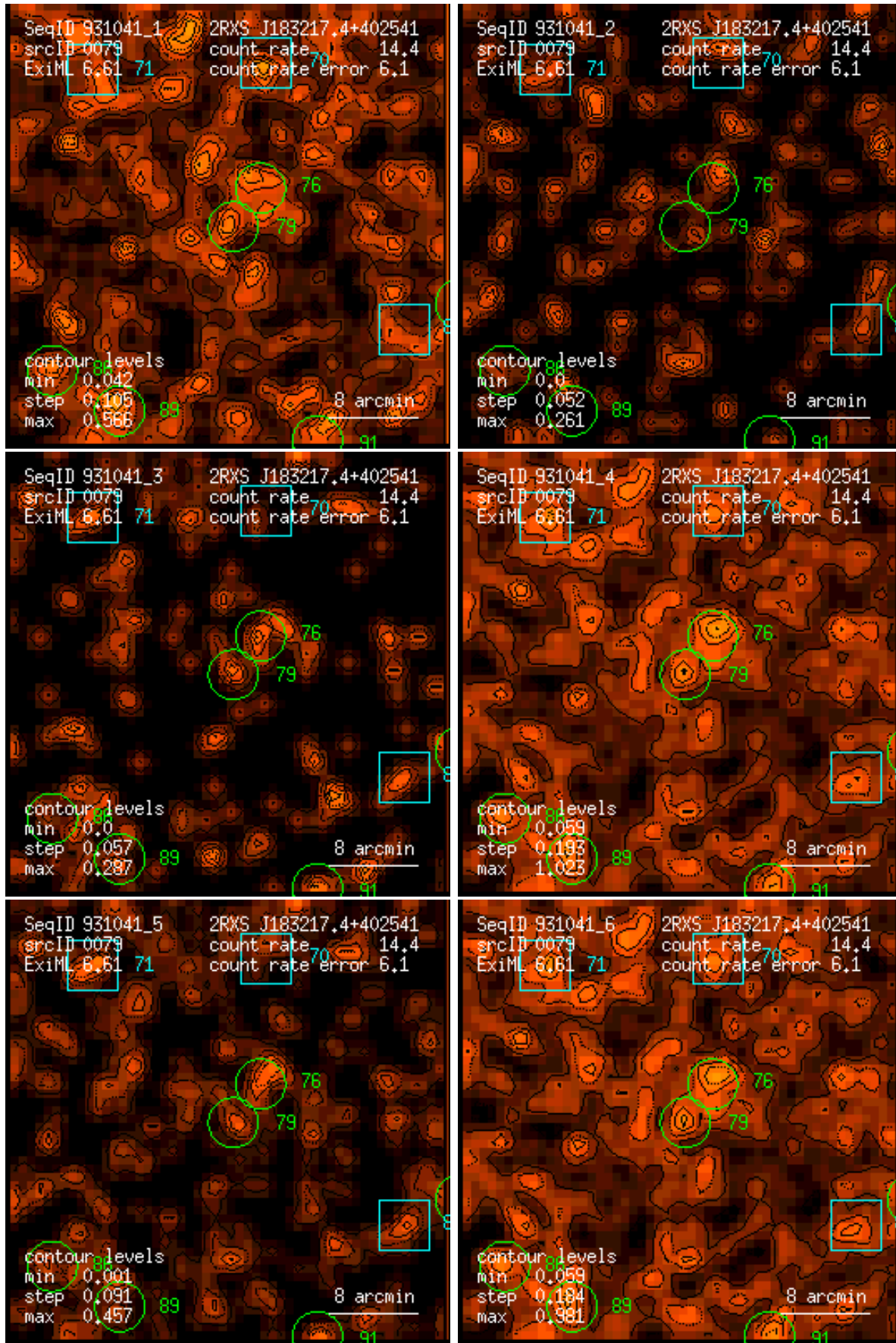
Figure 79: RASS 931041: detection 0079: band rate images, Gaussian filter: (1) PSPC channels 11 – 41, (2) 52 – 90, (3) 91 – 201, (4) 11 – 235, (5) 52 – 201, (6) 11 – 201. Broad band rates in counts/ks. Band rate contour levels in counts/ks/arcmin 2 .
