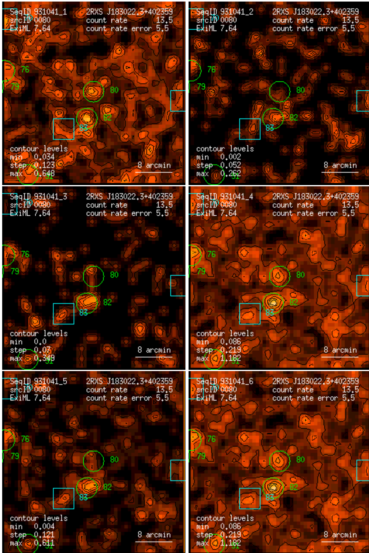
Figure 80: RASS 931041: detection 0080: band rate images, Gaussian filter: (1) PSPC channels 11 – 41, (2) 52 – 90, (3) 91 – 201, (4) 11 – 235, (5) 52 – 201, (6) 11 – 201. Broad band rates in counts/ks. Band rate contour levels in counts/ks/arcmin 2 .
