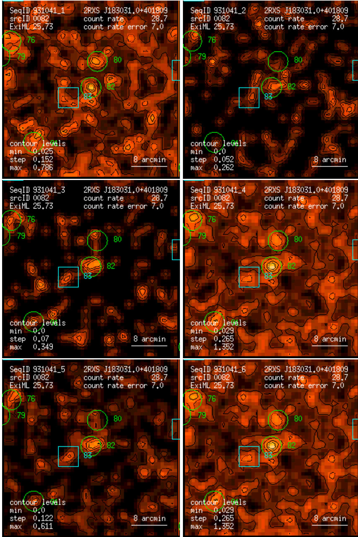
Figure 82: RASS 931041: detection 0082: band rate images, Gaussian filter: (1) PSPC channels 11 – 41, (2) 52 – 90, (3) 91 – 201, (4) 11 – 235, (5) 52 – 201, (6) 11 – 201. Broad band rates in counts/ks. Band rate contour levels in counts/ks/arcmin 2 .
