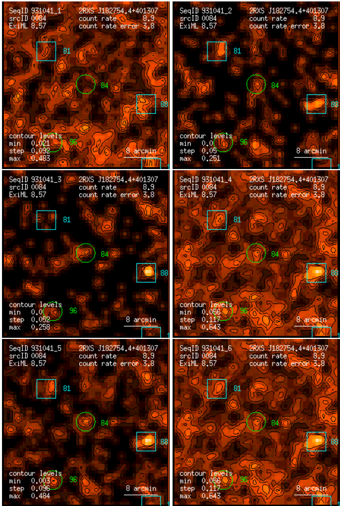
Figure 84: RASS 931041: detection 0084: band rate images, Gaussian filter: (1) PSPC channels 11 – 41, (2) 52 – 90, (3) 91 – 201, (4) 11 – 235, (5) 52 – 201, (6) 11 – 201. Broad band rates in counts/ks. Band rate contour levels in counts/ks/arcmin 2 .
