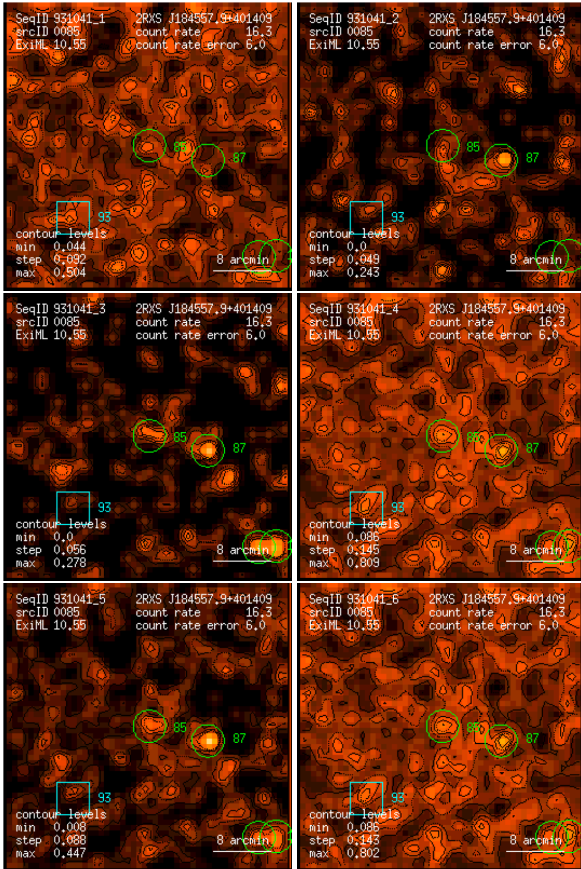
Figure 85: RASS 931041: detection 0085: band rate images, Gaussian filter: (1) PSPC channels 11 – 41, (2) 52 – 90, (3) 91 – 201, (4) 11 – 235, (5) 52 – 201, (6) 11 – 201. Broad band rates in counts/ks. Band rate contour levels in counts/ks/arcmin 2 .
