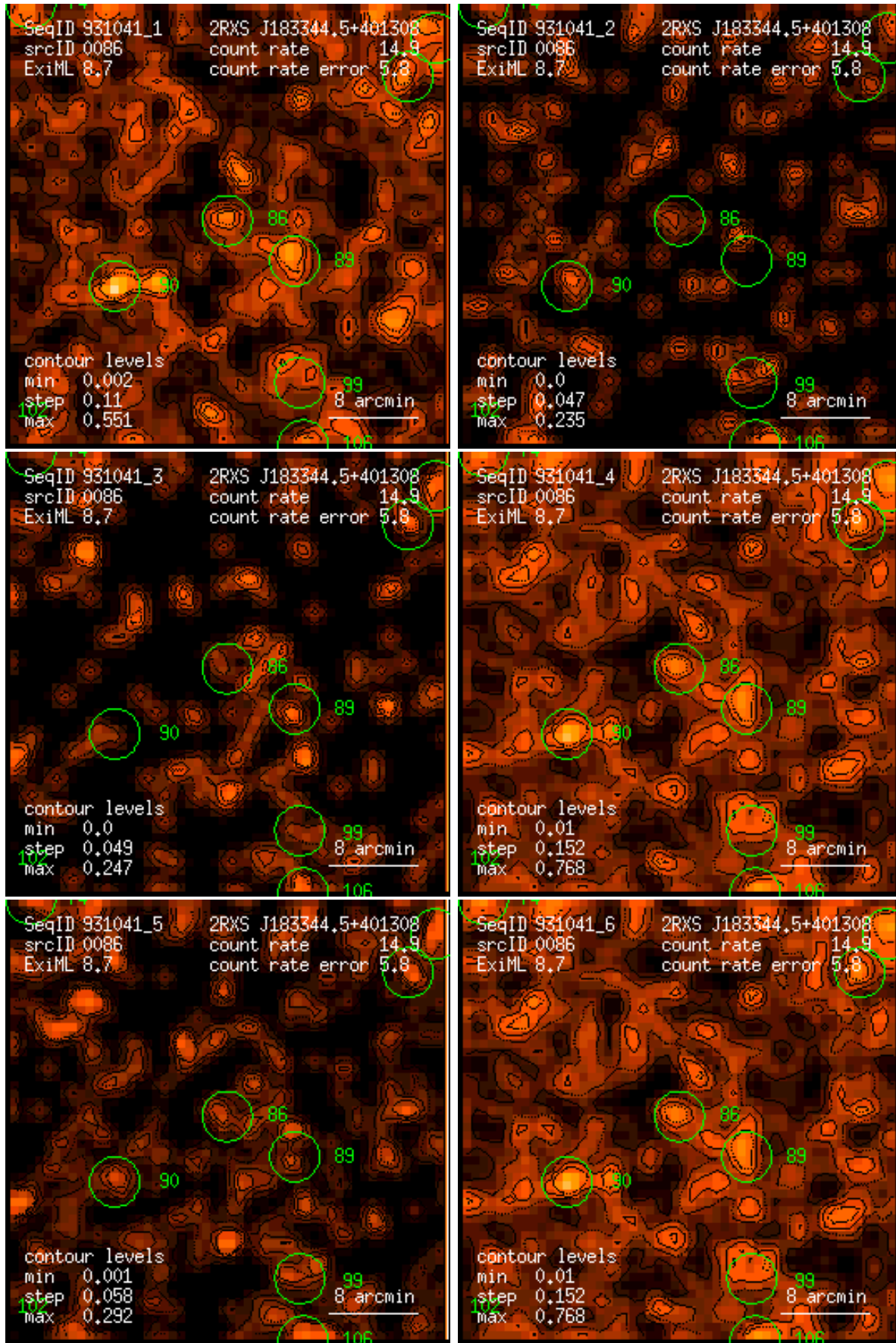
Figure 86: RASS 931041: detection 0086: band rate images, Gaussian filter: (1) PSPC channels 11 – 41, (2) 52 – 90, (3) 91 – 201, (4) 11 – 235, (5) 52 – 201, (6) 11 – 201. Broad band rates in counts/ks. Band rate contour levels in counts/ks/arcmin 2 .
