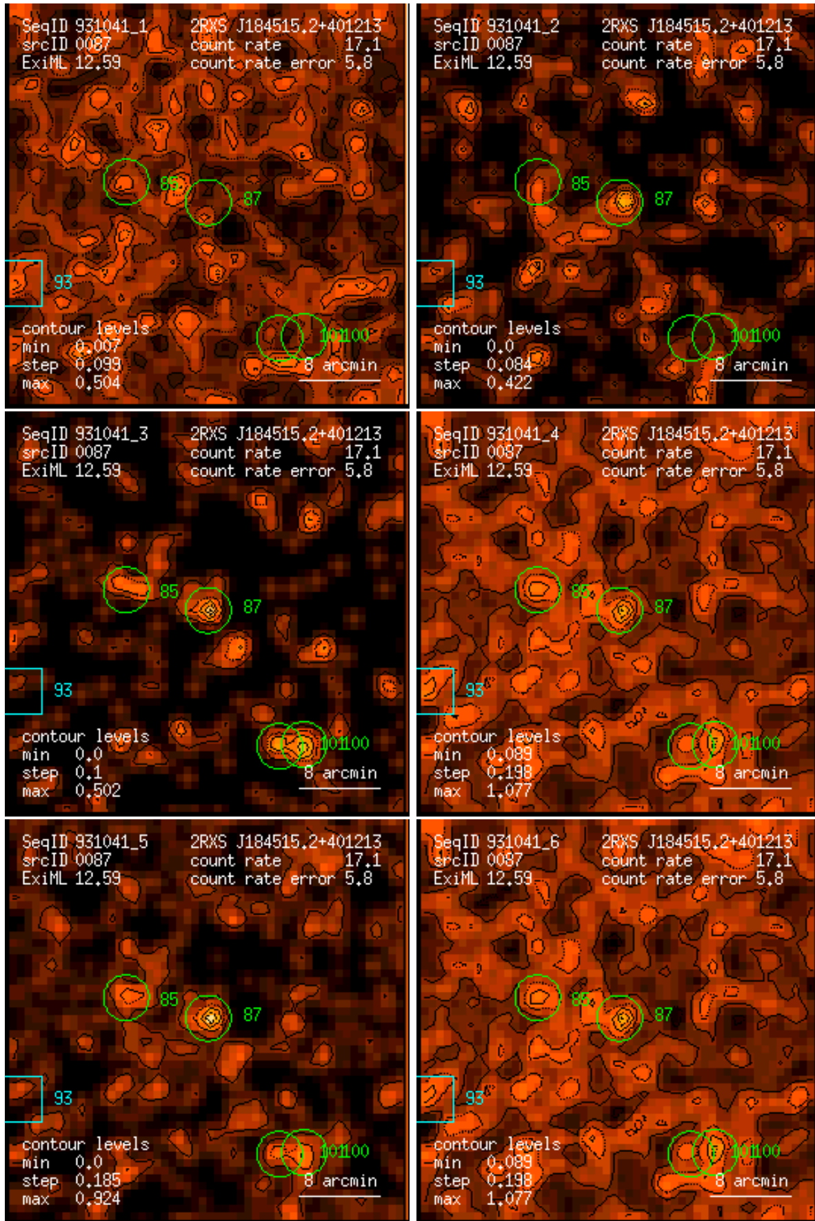
Figure 87: RASS 931041: detection 0087: band rate images, Gaussian filter: (1) PSPC channels 11 – 41, (2) 52 – 90, (3) 91 – 201, (4) 11 – 235, (5) 52 – 201, (6) 11 – 201. Broad band rates in counts/ks. Band rate contour levels in counts/ks/arcmin 2 .
