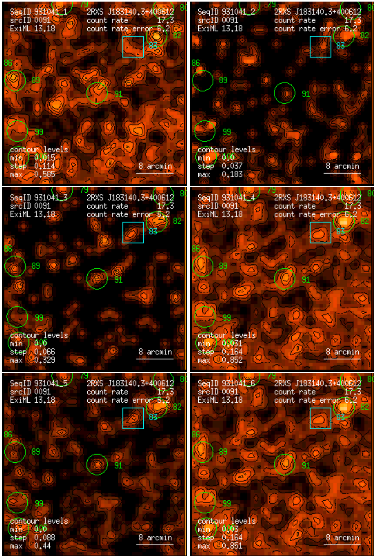
Figure 91: RASS 931041: detection 0091: band rate images, Gaussian filter: (1) PSPC channels 11 – 41, (2) 52 – 90, (3) 91 – 201, (4) 11 – 235, (5) 52 – 201, (6) 11 – 201. Broad band rates in counts/ks. Band rate contour levels in counts/ks/arcmin 2 .
