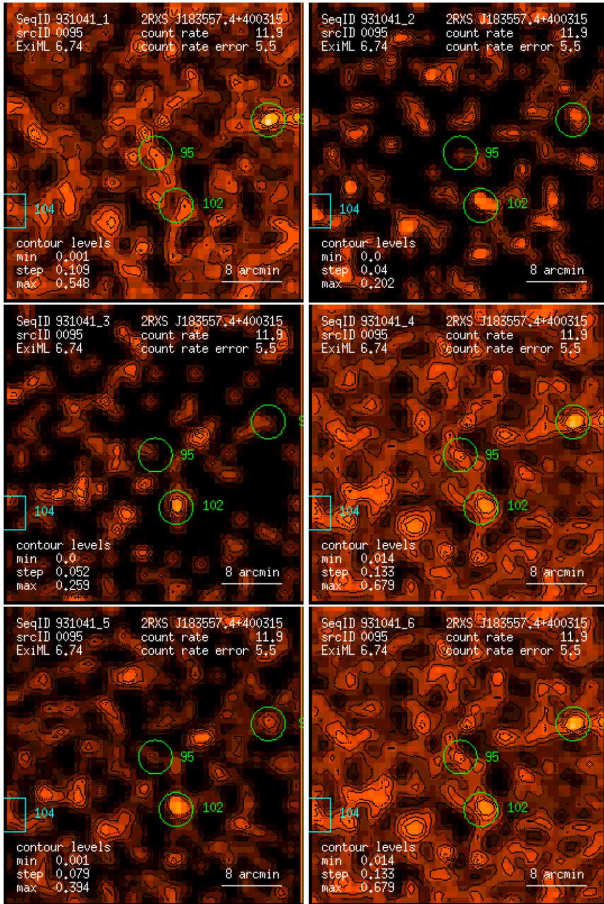
Figure 95: RASS 931041: detection 0095: band rate images, Gaussian filter: (1) PSPC channels 11 – 41, (2) 52 – 90, (3) 91 – 201, (4) 11 – 235, (5) 52 – 201, (6) 11 – 201. Broad band rates in counts/ks. Band rate contour levels in counts/ks/arcmin 2 .
