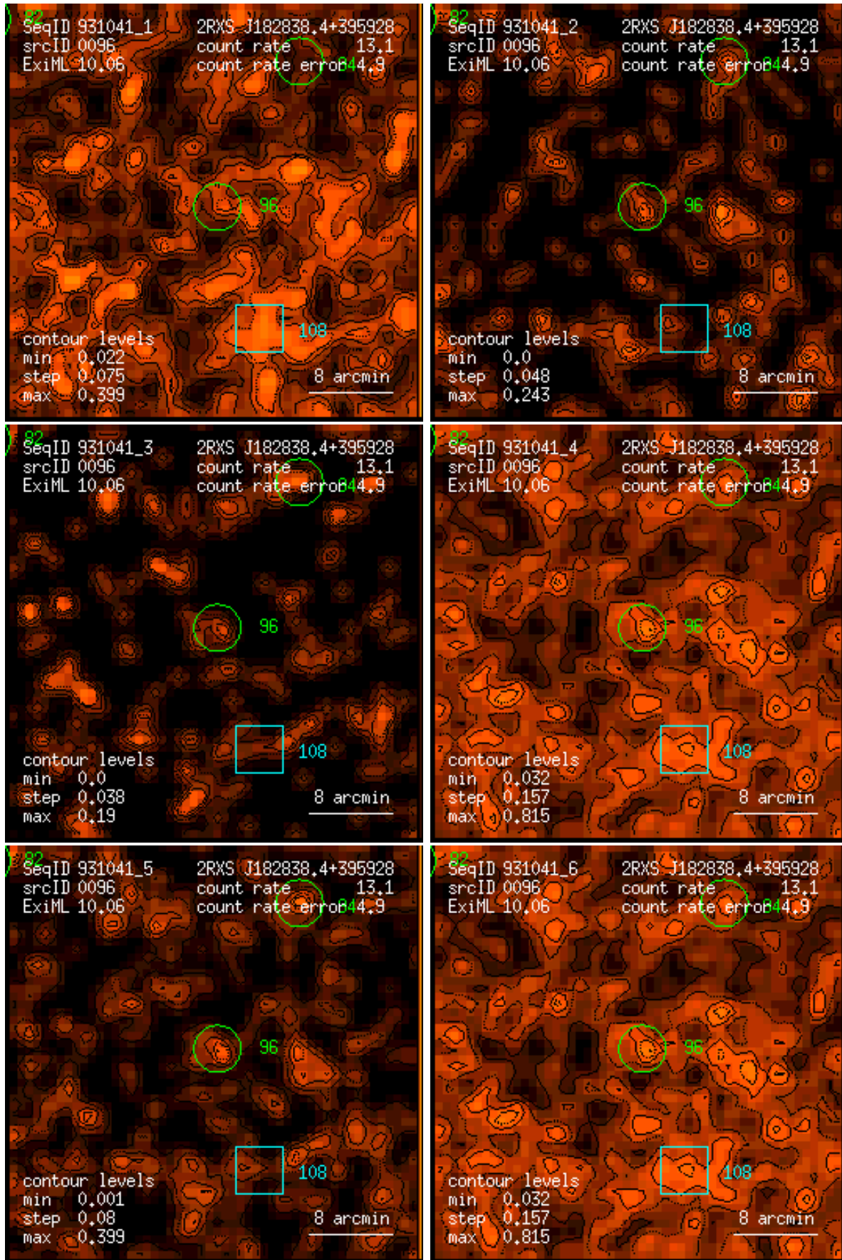
Figure 96: RASS 931041: detection 0096: band rate images, Gaussian filter: (1) PSPC channels 11 – 41, (2) 52 – 90, (3) 91 – 201, (4) 11 – 235, (5) 52 – 201, (6) 11 – 201. Broad band rates in counts/ks. Band rate contour levels in counts/ks/arcmin 2 .
