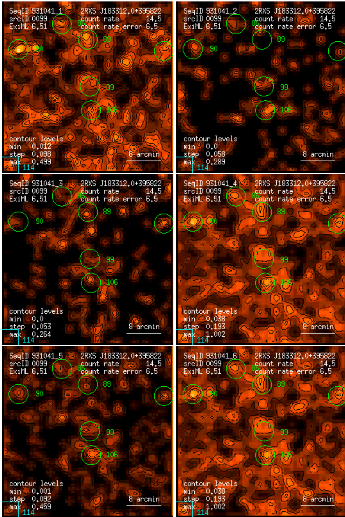
Figure 99: RASS 931041: detection 0099: band rate images, Gaussian filter: (1) PSPC channels 11 – 41, (2) 52 – 90, (3) 91 – 201, (4) 11 – 235, (5) 52 – 201, (6) 11 – 201. Broad band rates in counts/ks. Band rate contour levels in counts/ks/arcmin 2 .
