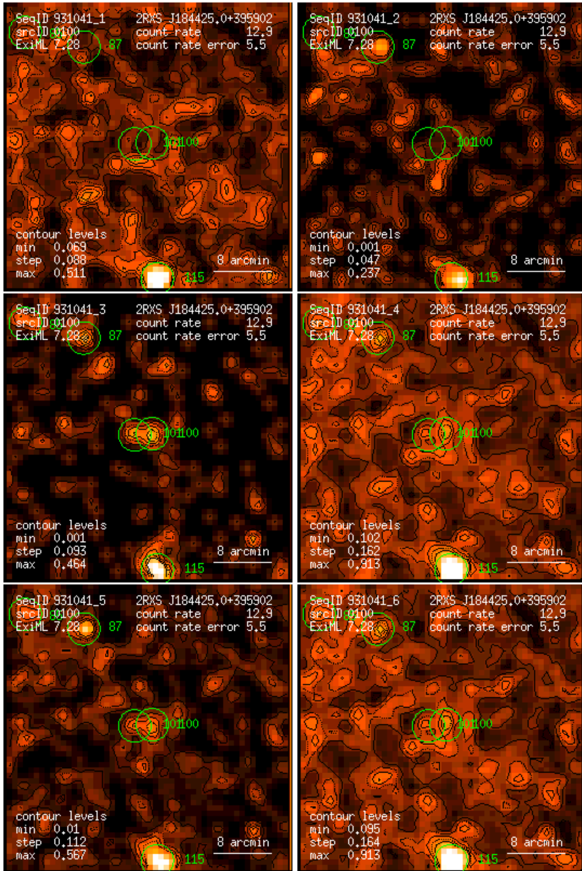
Figure 100: RASS 931041: detection 0100: band rate images, Gaussian filter: (1) PSPC channels 11 – 41, (2) 52 – 90, (3) 91 – 201, (4) 11 – 235, (5) 52 – 201, (6) 11 – 201. Broad band rates in counts/ks. Band rate contour levels in counts/ks/arcmin 2 .
