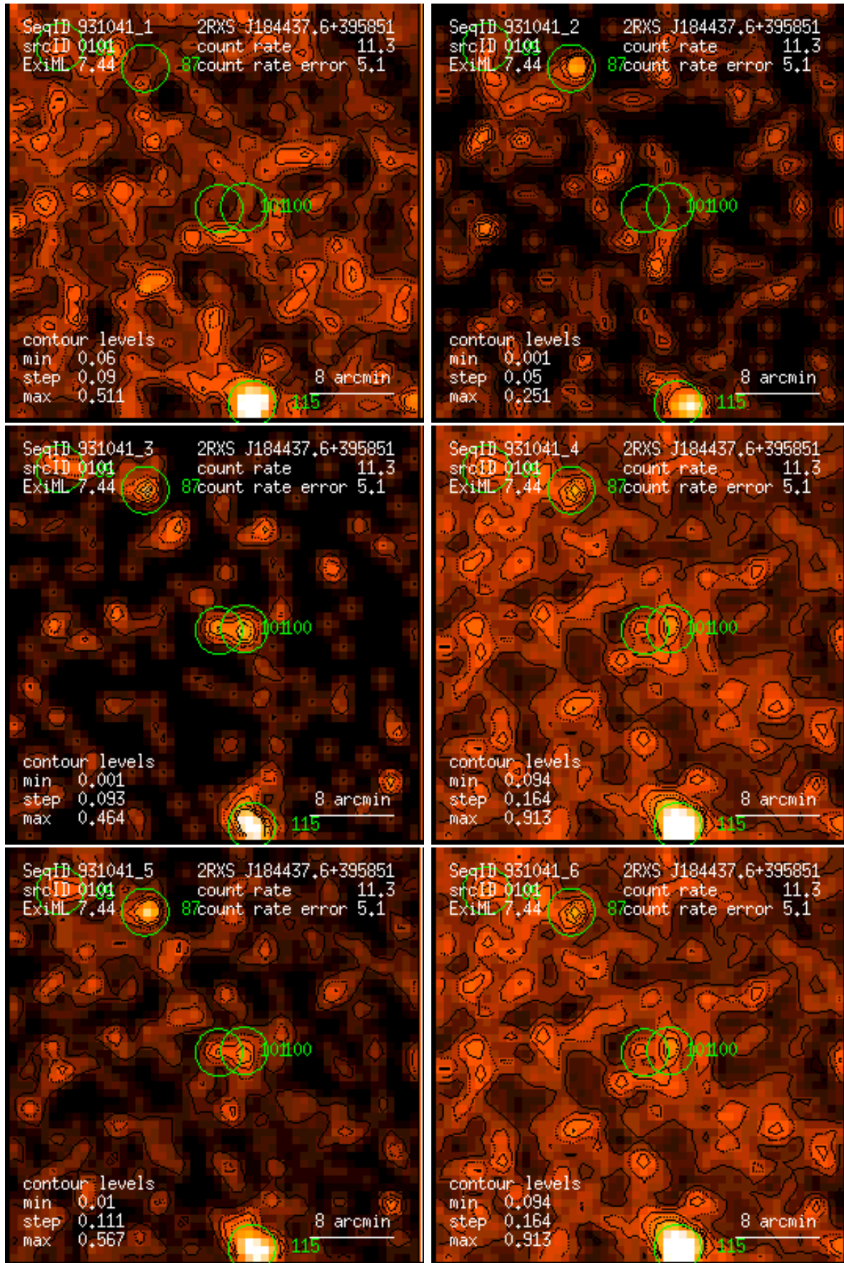
Figure 101: RASS 931041: detection 0101: band rate images, Gaussian filter: (1) PSPC channels 11 – 41, (2) 52 – 90, (3) 91 – 201, (4) 11 – 235, (5) 52 – 201, (6) 11 – 201. Broad band rates in counts/ks. Band rate contour levels in counts/ks/arcmin 2 .
