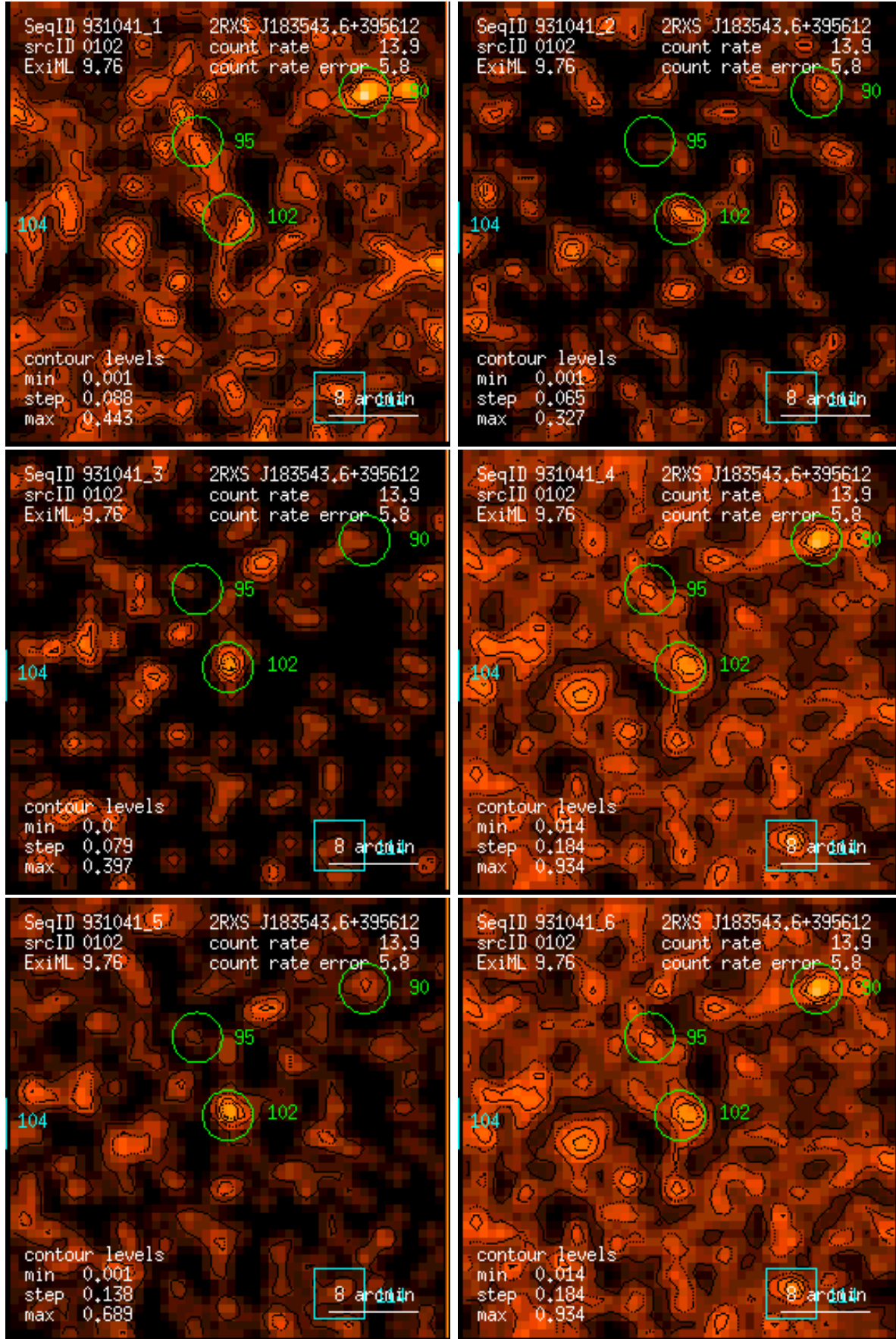
Figure 102: RASS 931041: detection 0102: band rate images, Gaussian filter: (1) PSPC channels 11 – 41, (2) 52 – 90, (3) 91 – 201, (4) 11 – 235, (5) 52 – 201, (6) 11 – 201. Broad band rates in counts/ks. Band rate contour levels in counts/ks/arcmin 2 .
