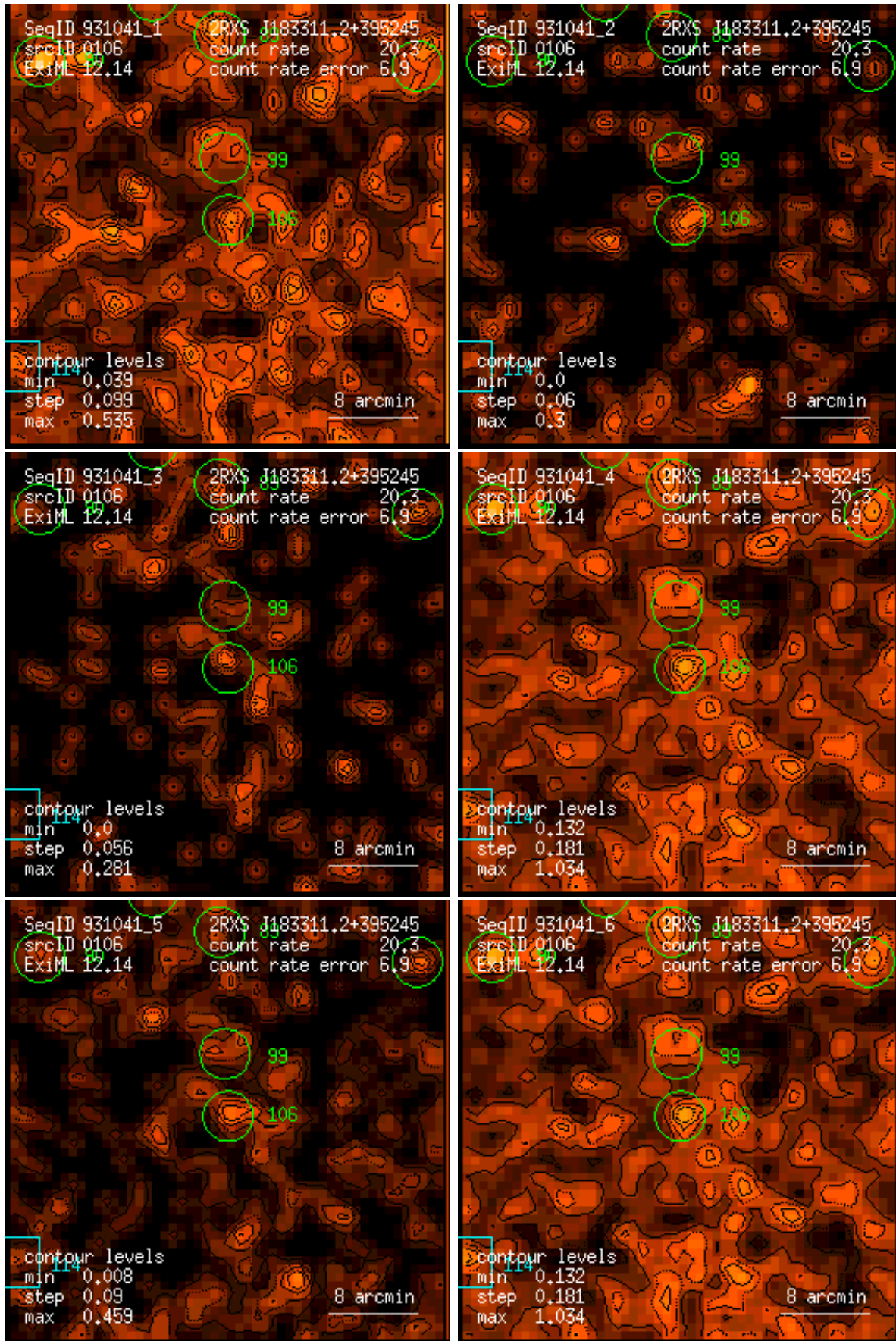
Figure 106: RASS 931041: detection 0106: band rate images, Gaussian filter: (1) PSPC channels 11 – 41, (2) 52 – 90, (3) 91 – 201, (4) 11 – 235, (5) 52 – 201, (6) 11 – 201. Broad band rates in counts/ks. Band rate contour levels in counts/ks/arcmin 2 .
