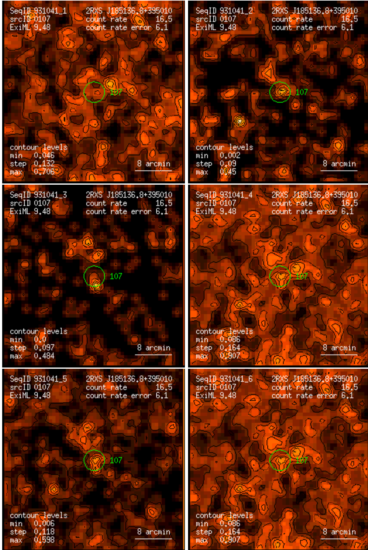
Figure 107: RASS 931041: detection 0107: band rate images, Gaussian filter: (1) PSPC channels 11 – 41, (2) 52 – 90, (3) 91 – 201, (4) 11 – 235, (5) 52 – 201, (6) 11 – 201. Broad band rates in counts/ks. Band rate contour levels in counts/ks/arcmin 2 .
