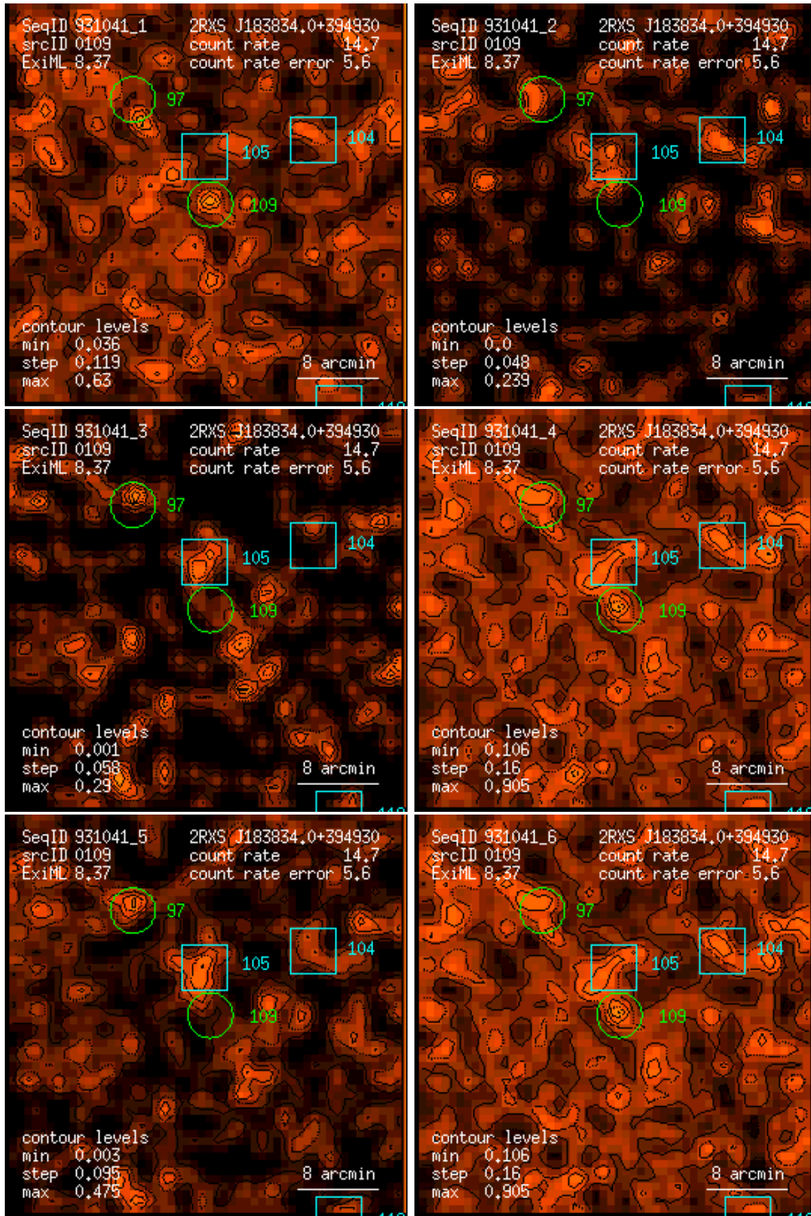
Figure 109: RASS 931041: detection 0109: band rate images, Gaussian filter: (1) PSPC channels 11 – 41, (2) 52 – 90, (3) 91 – 201, (4) 11 – 235, (5) 52 – 201, (6) 11 – 201. Broad band rates in counts/ks. Band rate contour levels in counts/ks/arcmin 2 .
