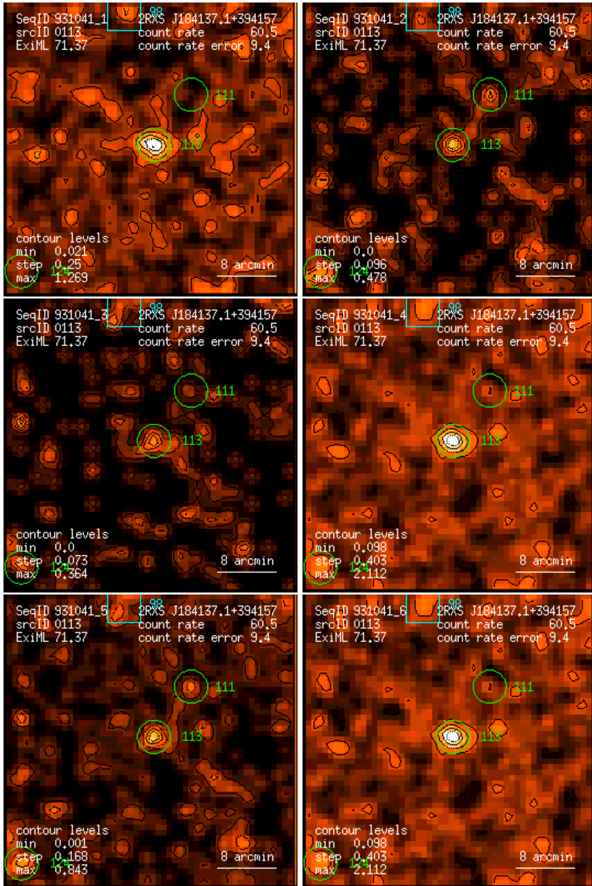
Figure 113: RASS 931041: detection 0113: band rate images, Gaussian filter: (1) PSPC channels 11 – 41, (2) 52 – 90, (3) 91 – 201, (4) 11 – 235, (5) 52 – 201, (6) 11 – 201. Broad band rates in counts/ks. Band rate contour levels in counts/ks/arcmin 2 .
